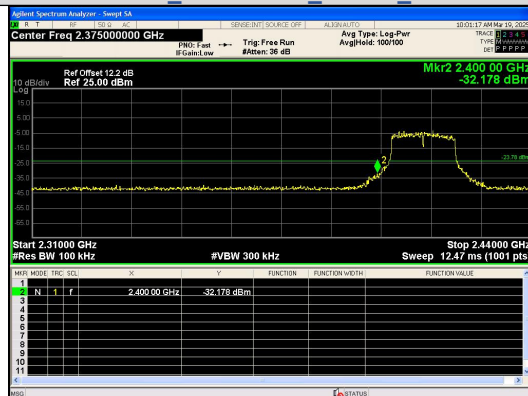
Out Of Band Emission IEEE 802.11q Channel 1 20MHz Antenna 0
