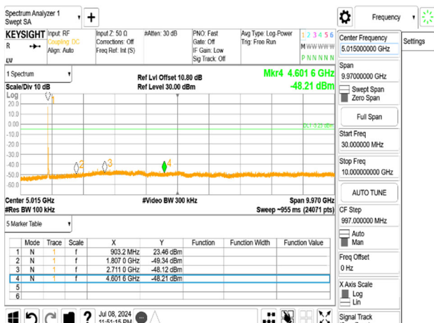
OFDM_1M_LowCH-903.5
