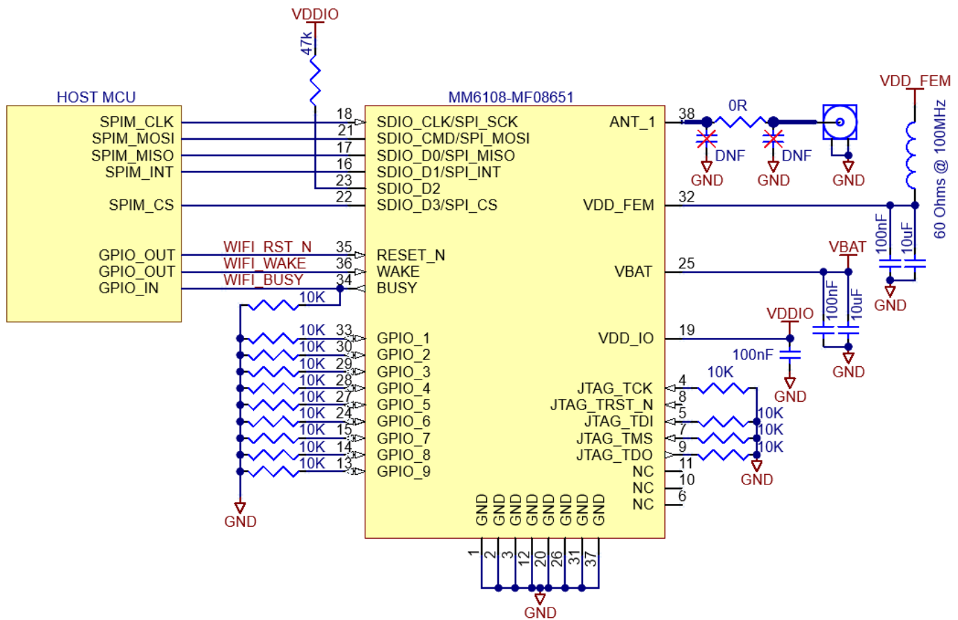
SPI Configuration
