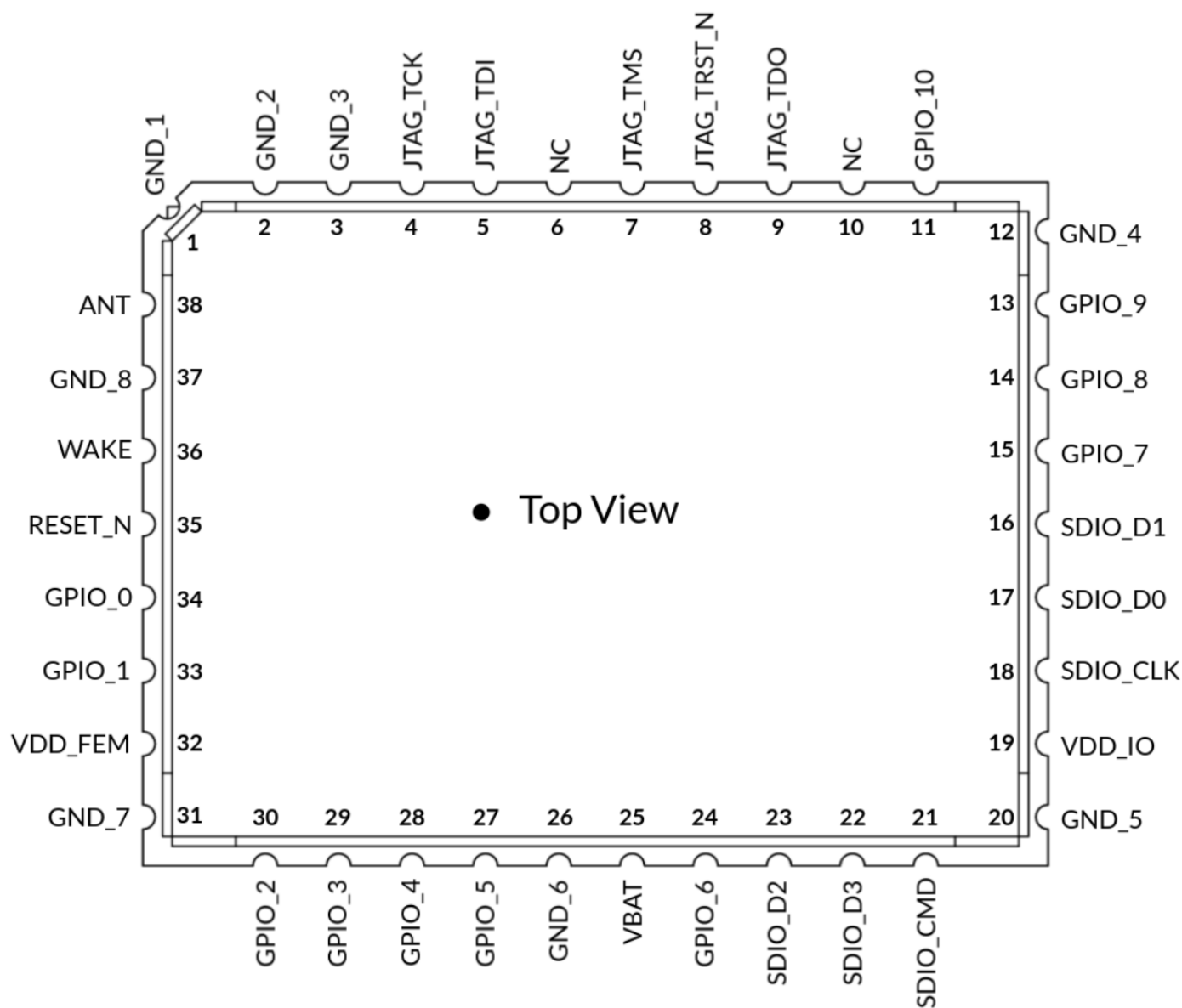
Figure 1: Pin Diagram
