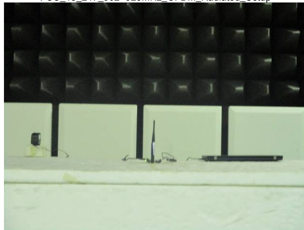
FCC_15_247_902~928MHz_OFDM_Radiated_Setup
