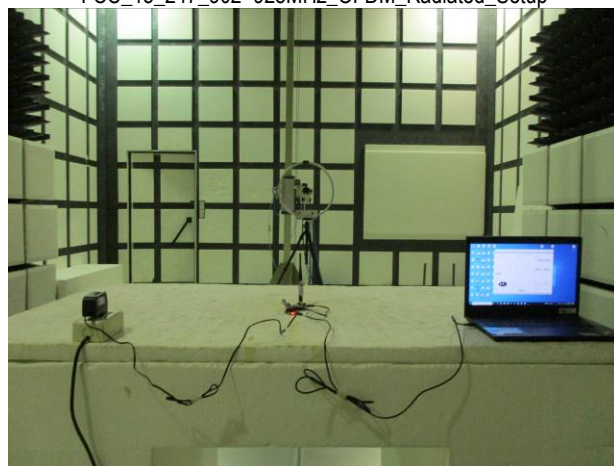
FCC_15_247_902~928MHz_OFDM_Radiated_Setup
