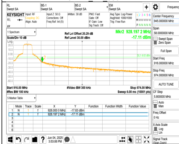
OFDM 4M 922MHz
