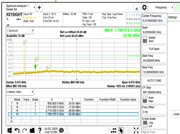
OFDM 2M 905MHz
