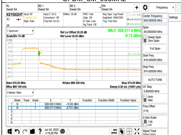
OFDM 8M 924MHz
