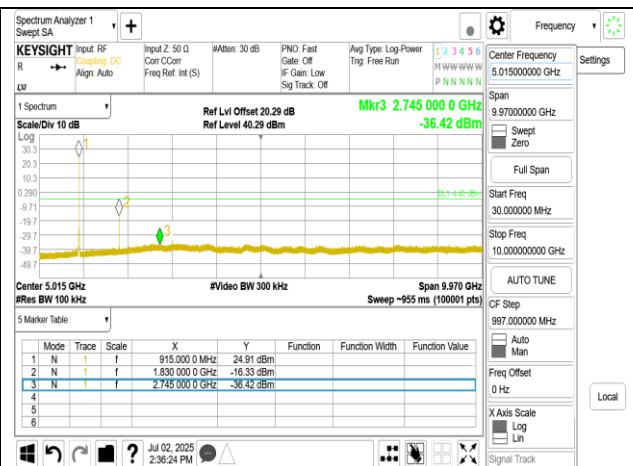
OFDM 2M 915MHz
