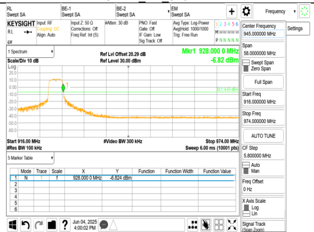
OFDM 4M 926MHz
