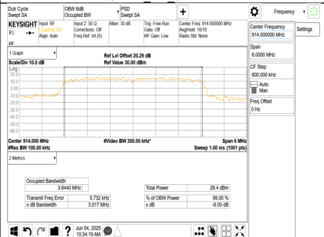
OFDM 4M 914MHz
