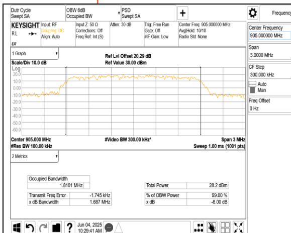
OFDM 2M 905MHz
