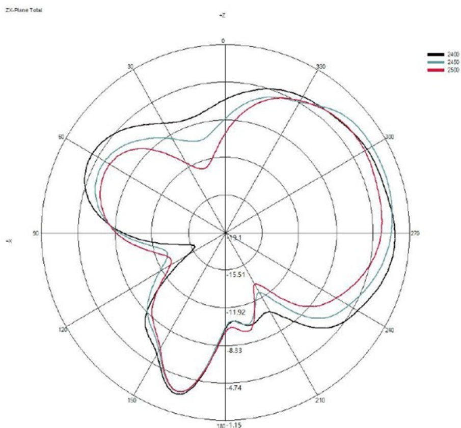
(1) X-Z Plane(unit:dBi):
