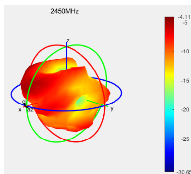
方向图、苹果图 (Directional and 3D diagram)
