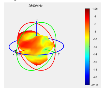
方向图、苹果图 (Directional and 3D diagram)
