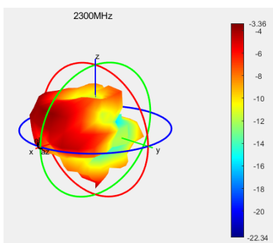
方向图、苹果图 (Directional and 3D diagram)
