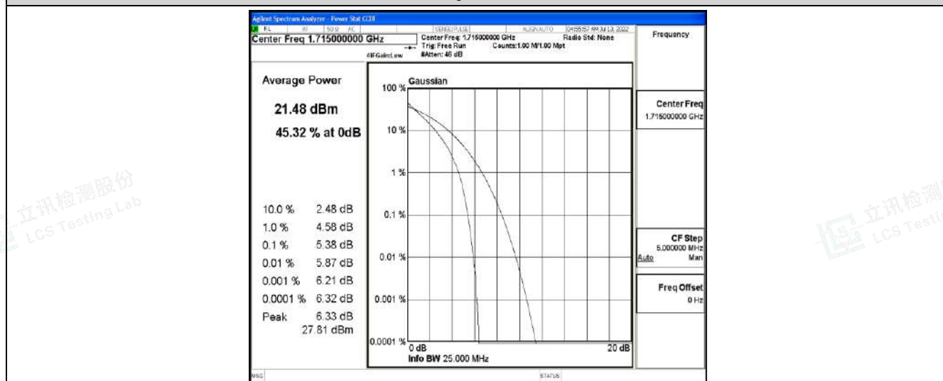
Band4-10MHz-QPSK-20175-50RB#0
