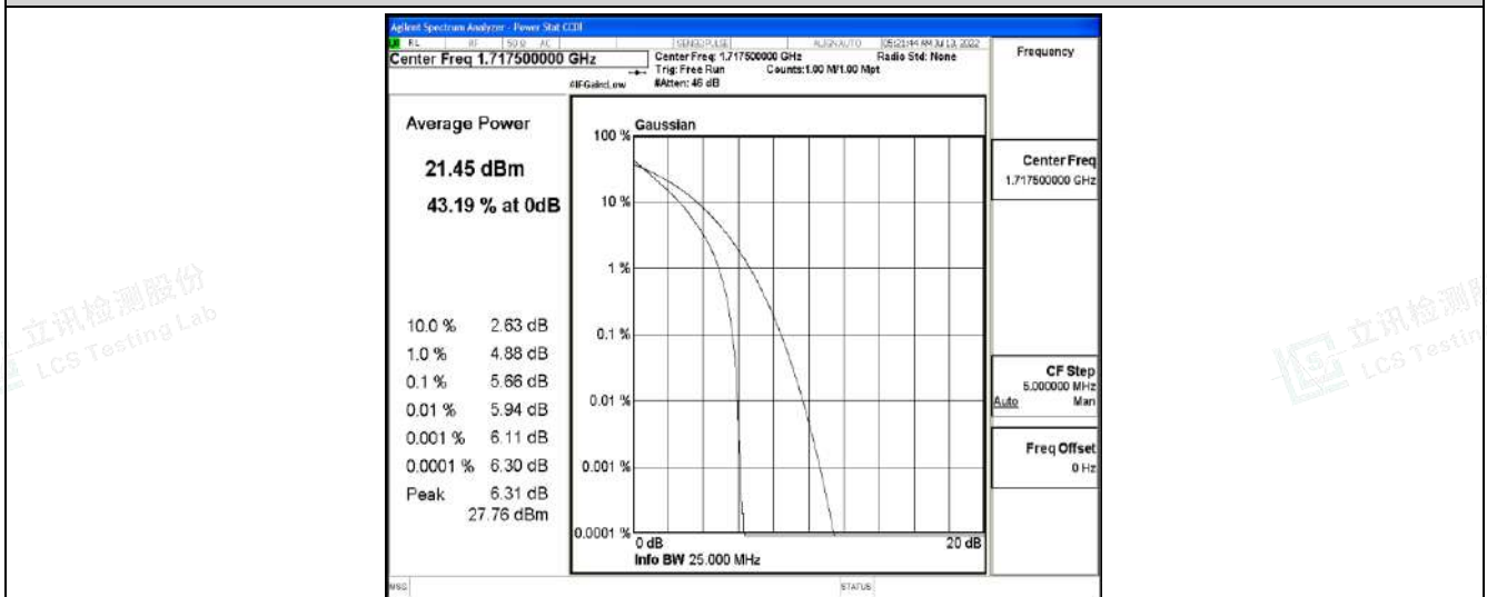
Band4-15MHz-QPSK-20175-75RB#0
