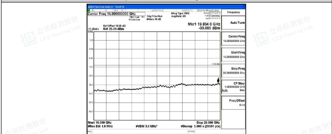
Band4-20MHz-16QAM-20300-1RB#0-Range5:10000~20000MHz
