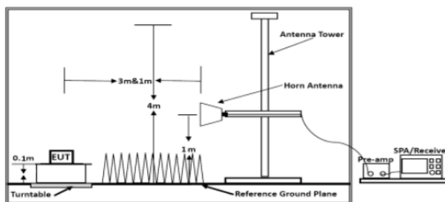
Figure 3. Above 1GHz
