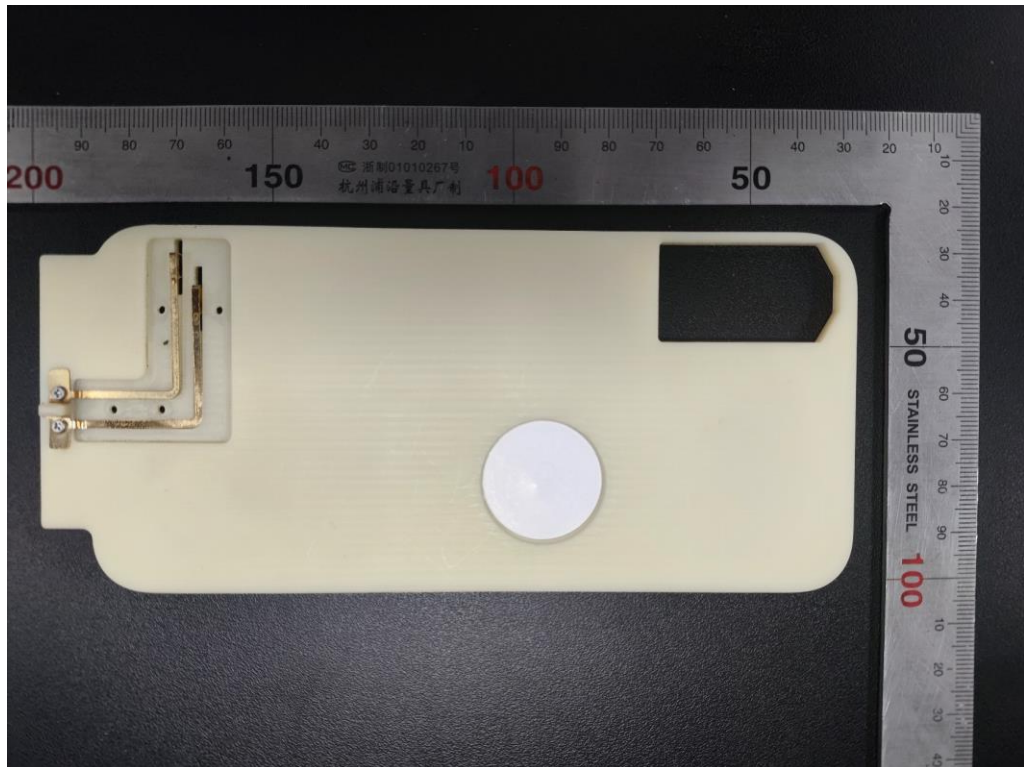
Photo 21: Interpoer plate
