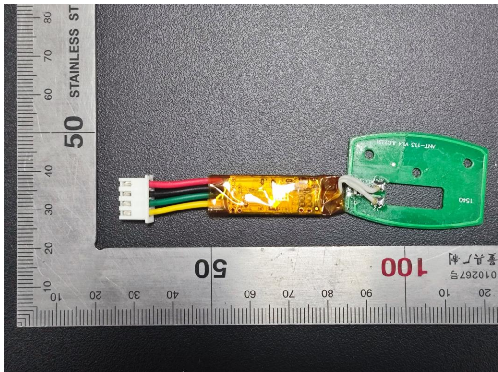
Photo 12: PCBA of the Charge plate
