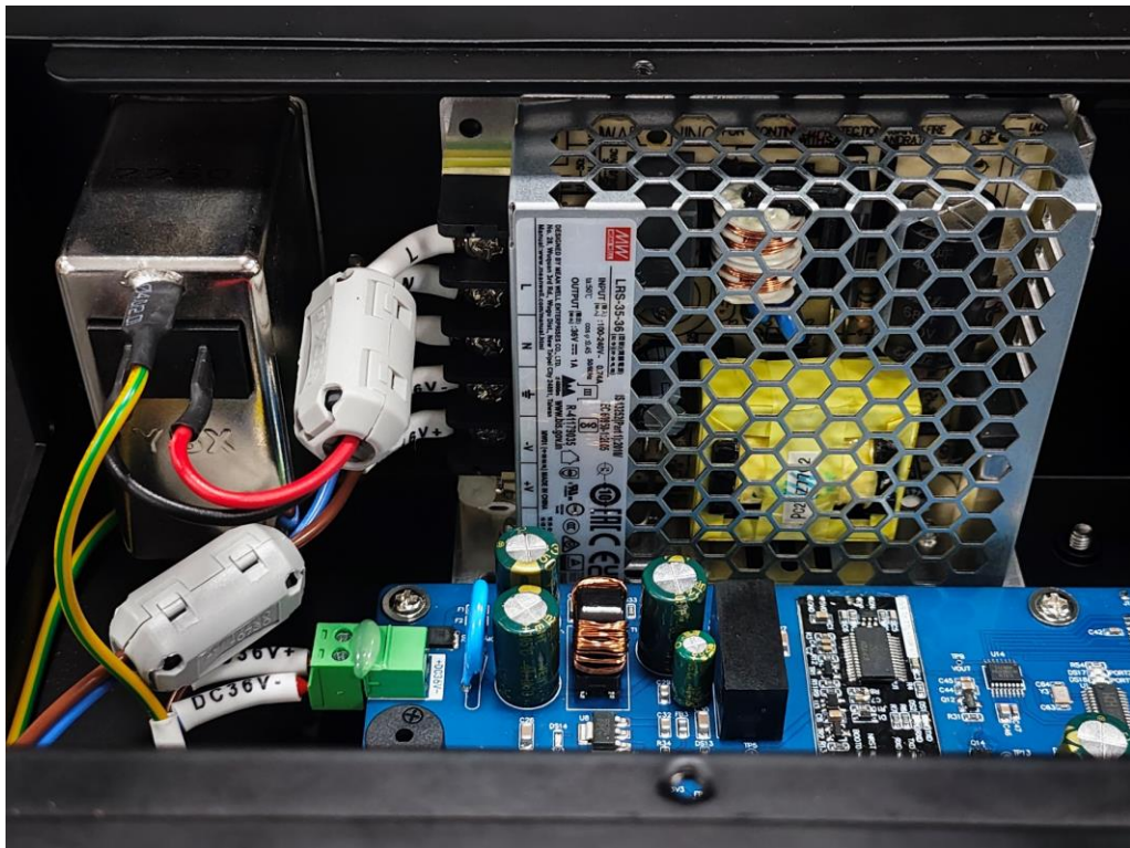
Photo 5: Internal view
