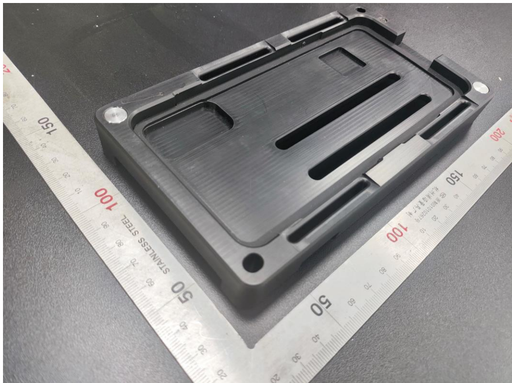
Photo 16: Overall view of the Repair sled
