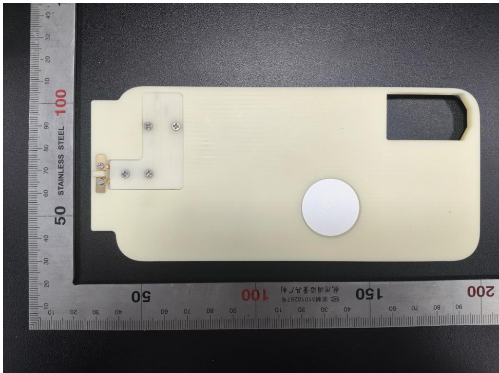
Photo 20: Interpoer plate
