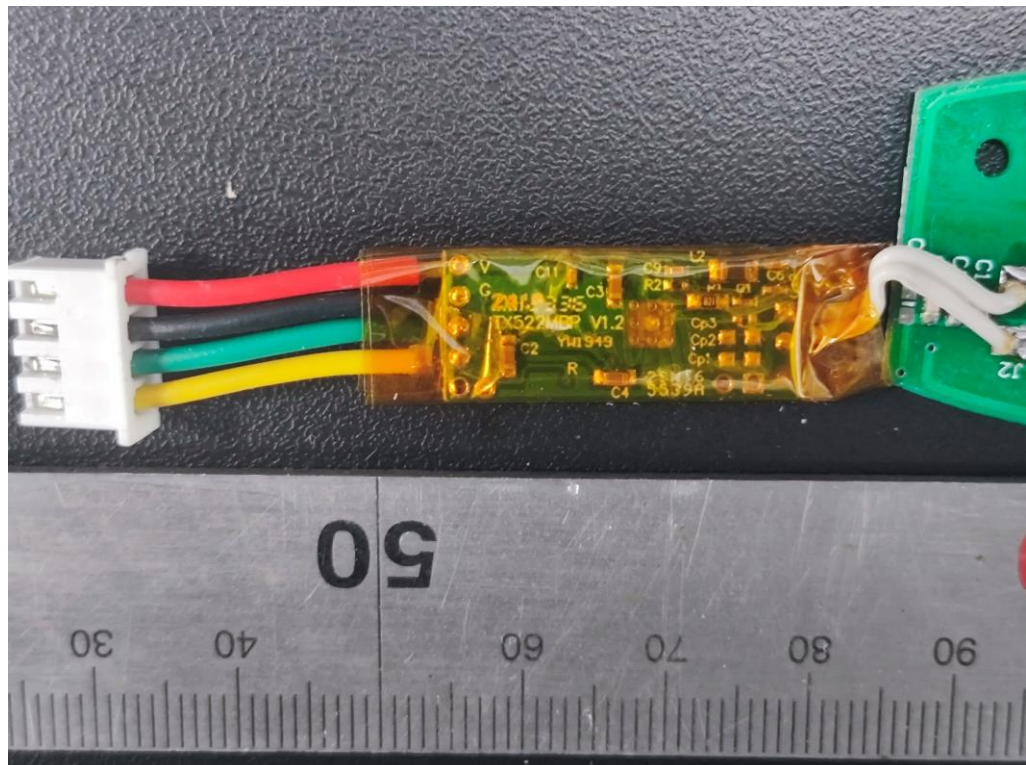
Photo 14: PCBA of the Charge plate
