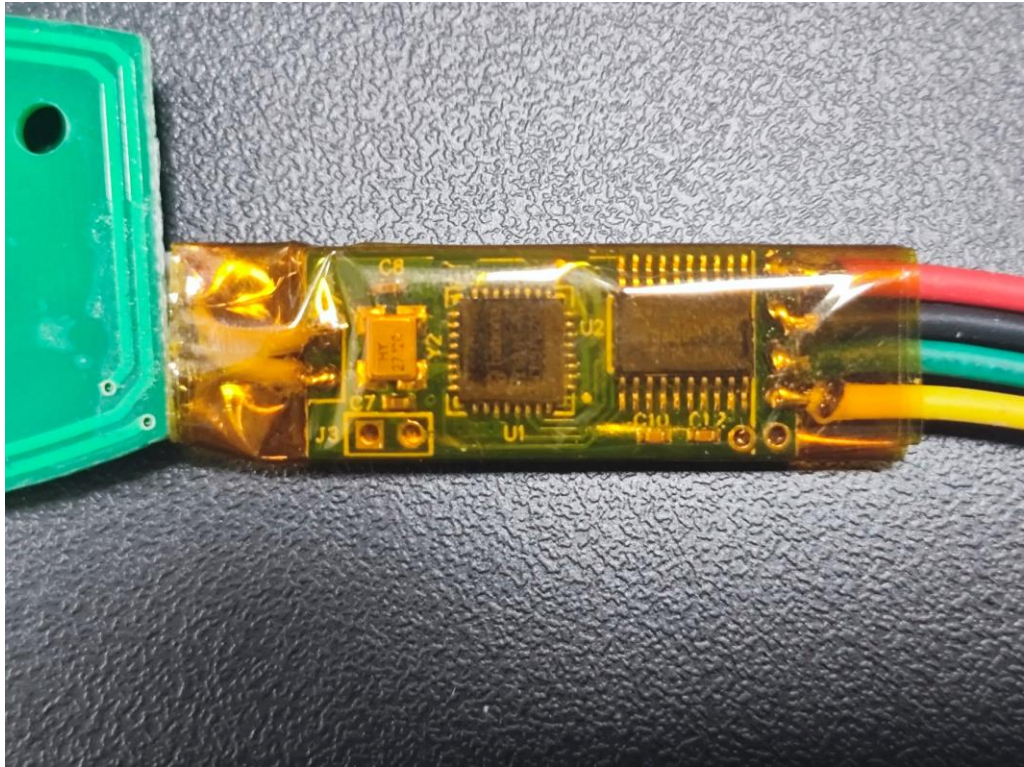
Photo 15: PCBA of the Charge plate
