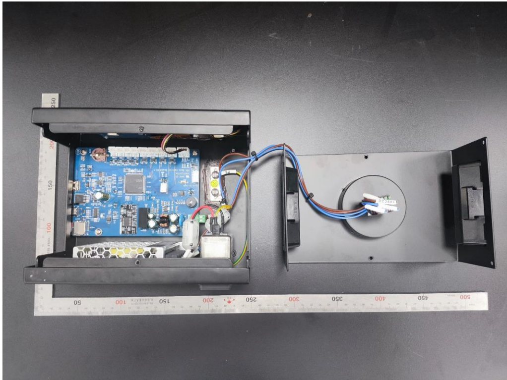
Photo 1: Internal view
