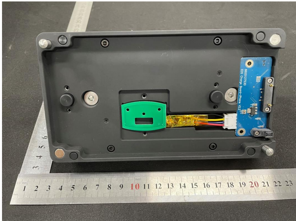
Photo 11: Internal view of the Charge plate
