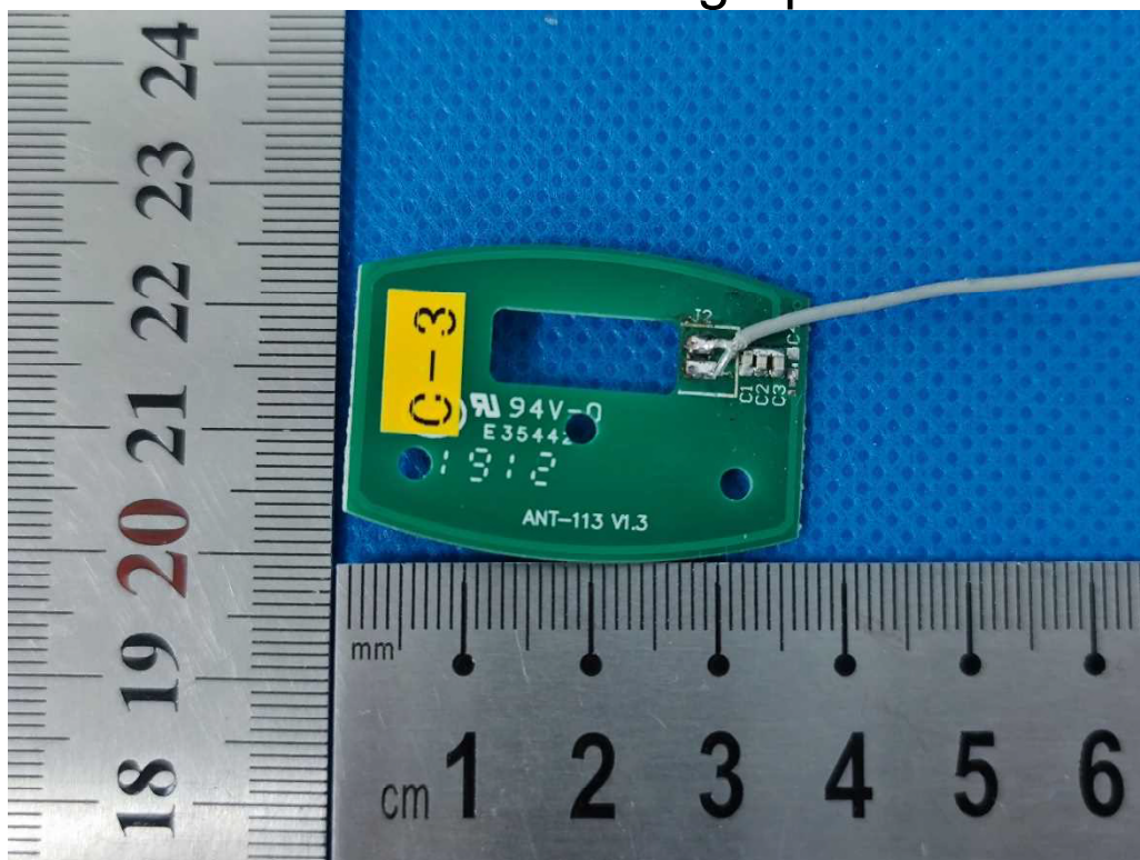
Antenna Photograph
