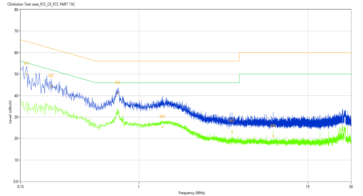
Figure 13: Conducted Emission on AC Mains, L Phase
