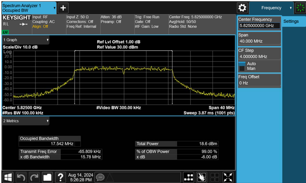
Figure 12: The plots of 6dB Bandwidth, 802.11n(HT20), 5825MHz
