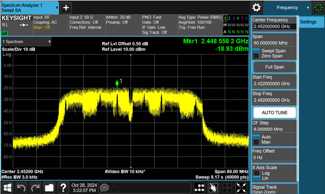
Figure 24: Power Spectral Density, 802.11n(H40), 2452MHz
