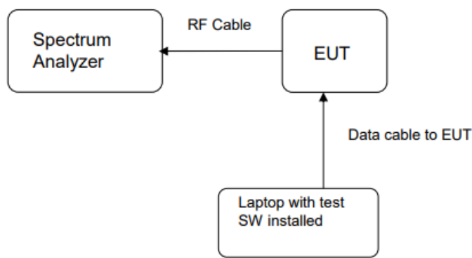
Diagram of Measurement Configuration for Conduction Test
