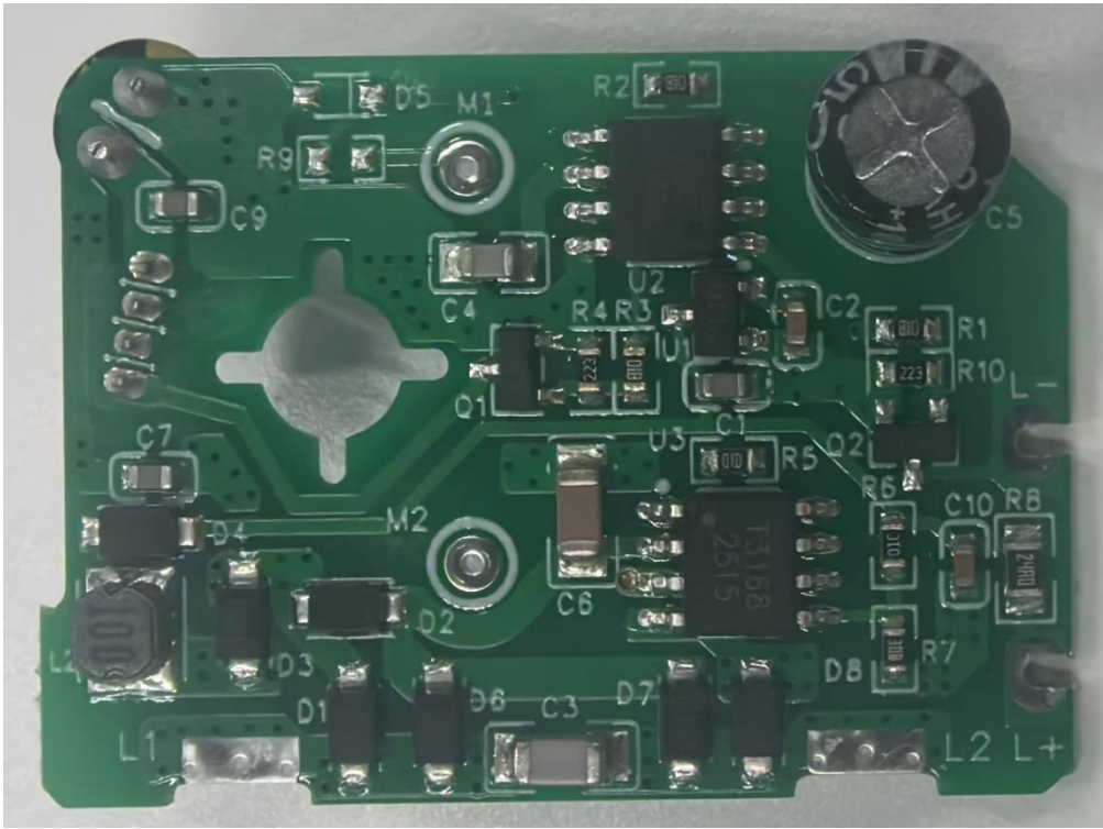
Wireless pump-PCB(Front)
