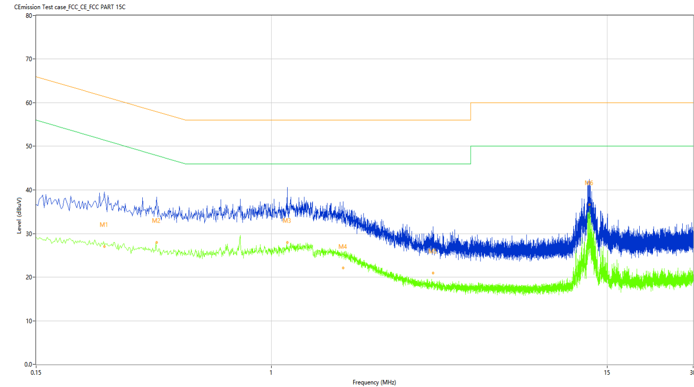
Figure 14: Conducted Emission on AC Mains, L Phase
