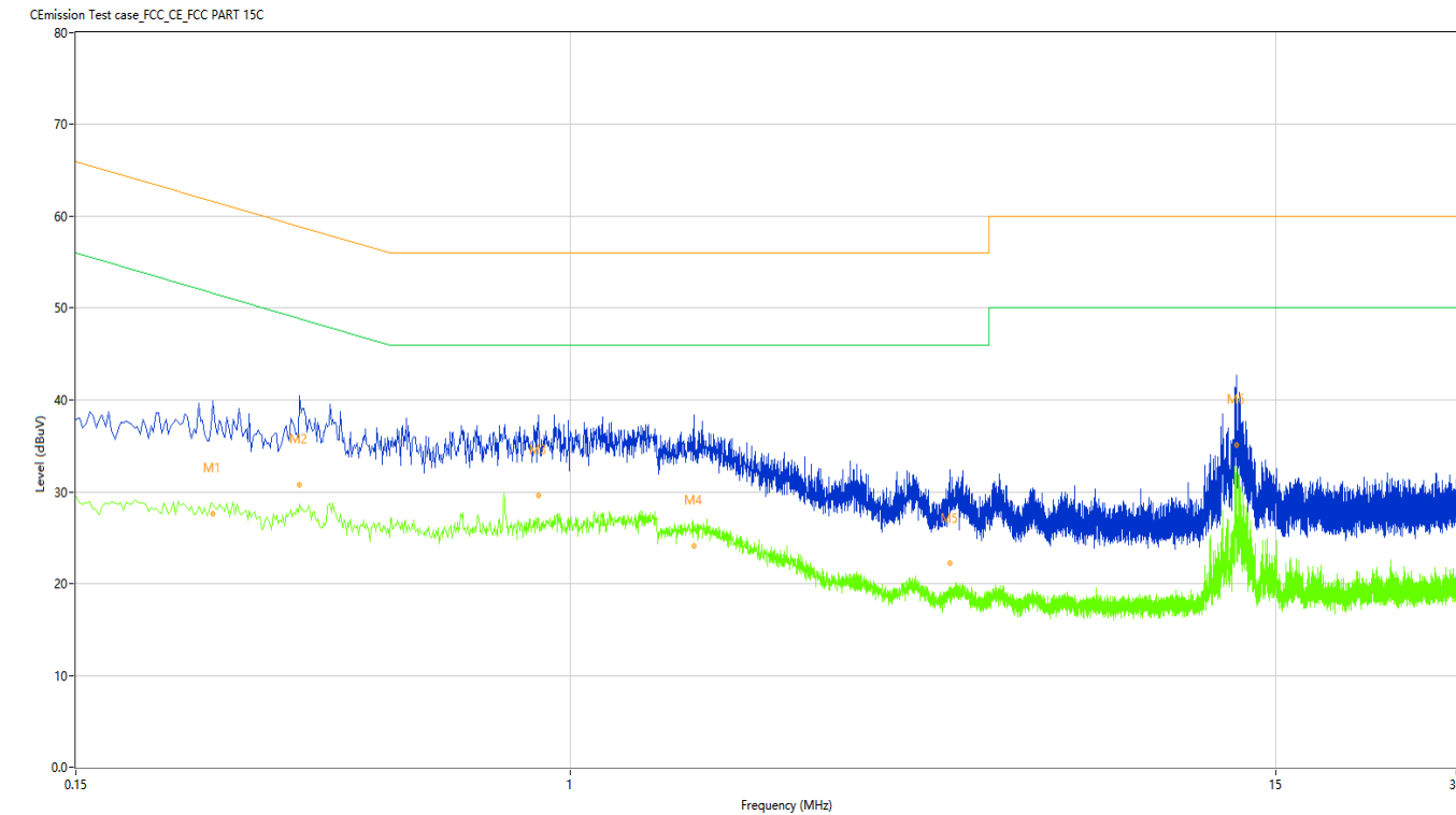
Figure 13: Conducted Emission on AC Mains, N Phase
