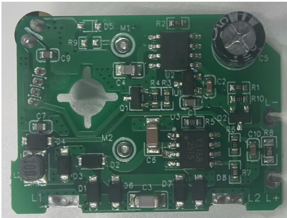
Wireless pump-PCB(Front)
