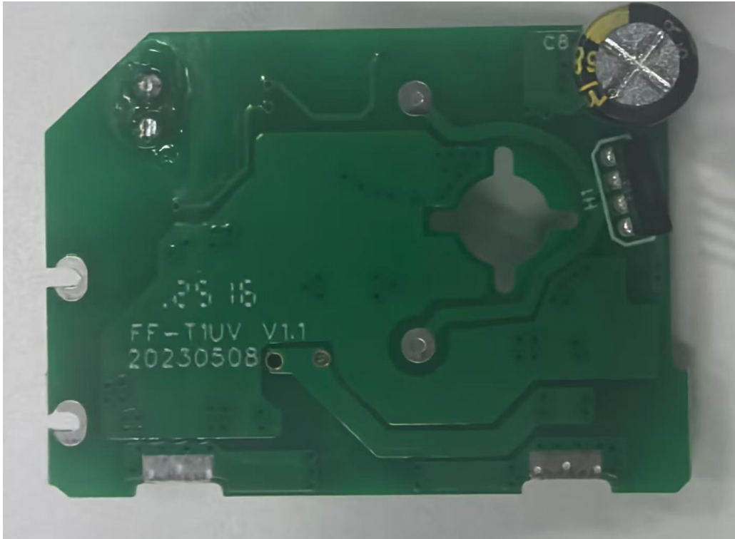
Wireless pump-PCB(Back)
