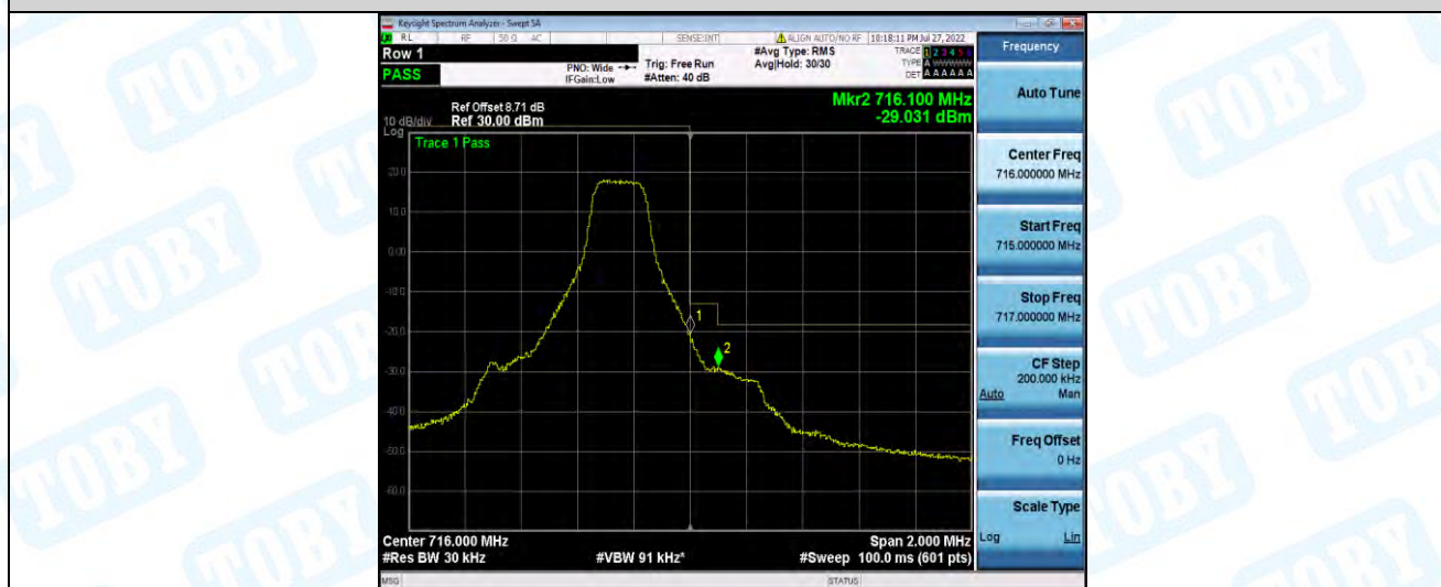
Band12-1.4MHz-QPSK-23173-6RB#0
