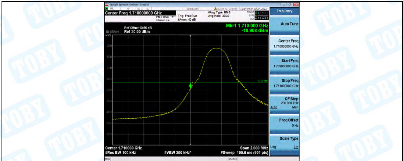
Band4-5MHz-QPSK-19975-1RB#24
