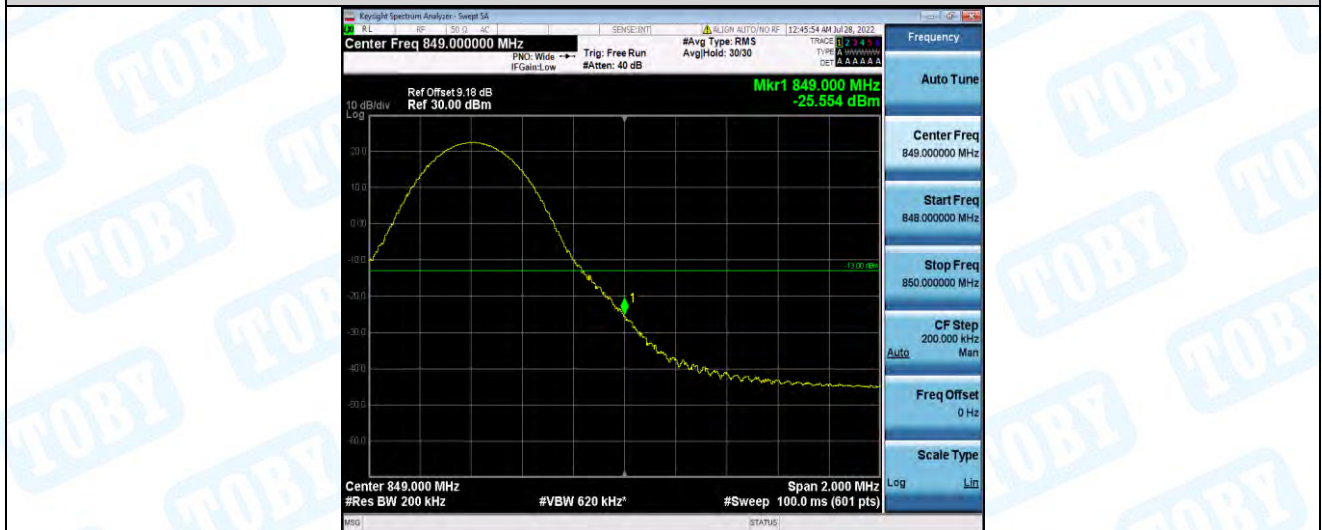
Band5-10MHz-QPSK-20600-50RB#0
