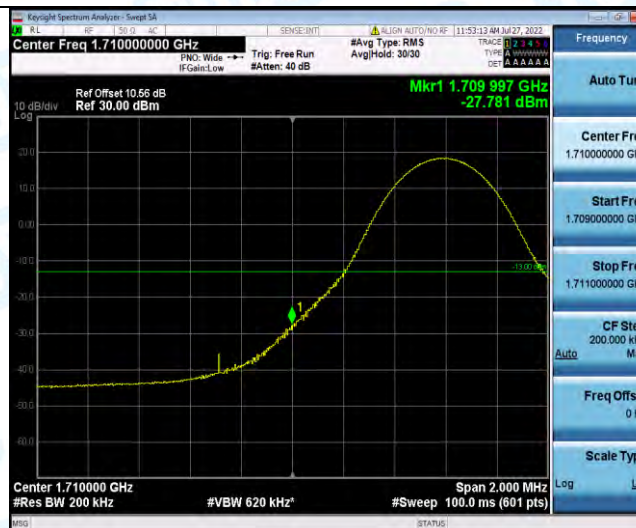
Band4-10MHz-16QAM-20000-1RB#49
