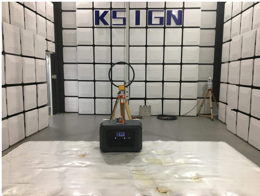
Radiated Measurement (Below 30MHz)
