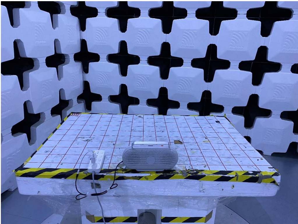
The EUT was placed at the center of turntable
