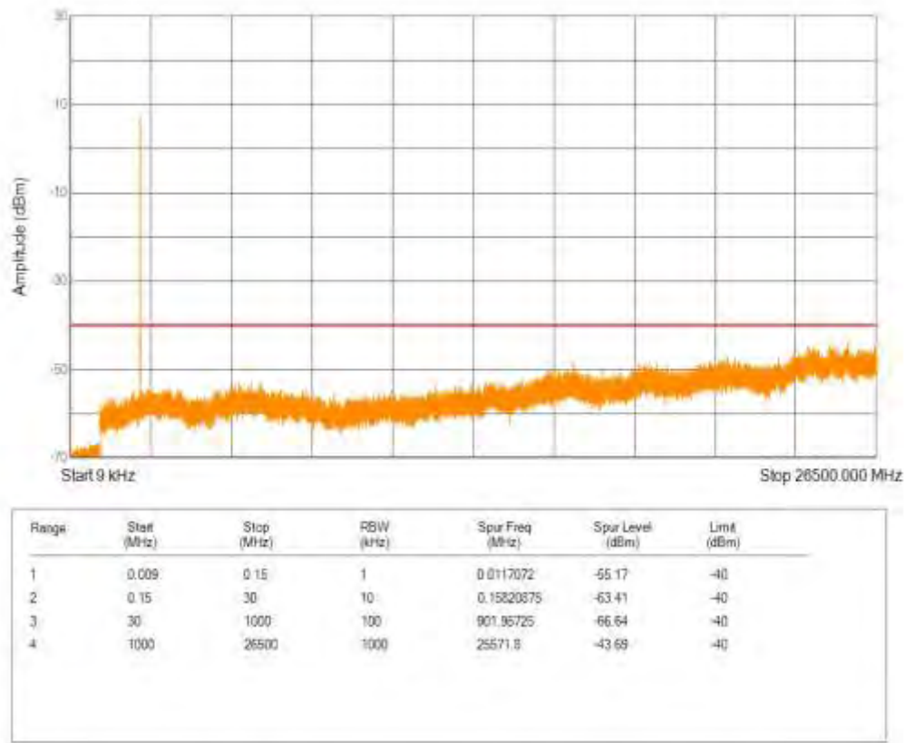
Band40(2350-2360) QAM16 BW=10MHz Channel=39200 RB Size=50 Position=#0
