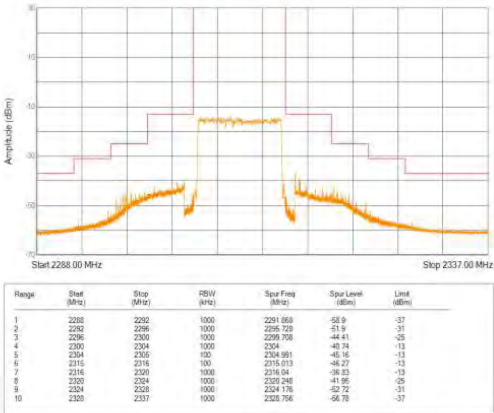
Band40(2305-2315) QAM16 BW=5MHz Channel=38725 RB Size=25 Position=#0
