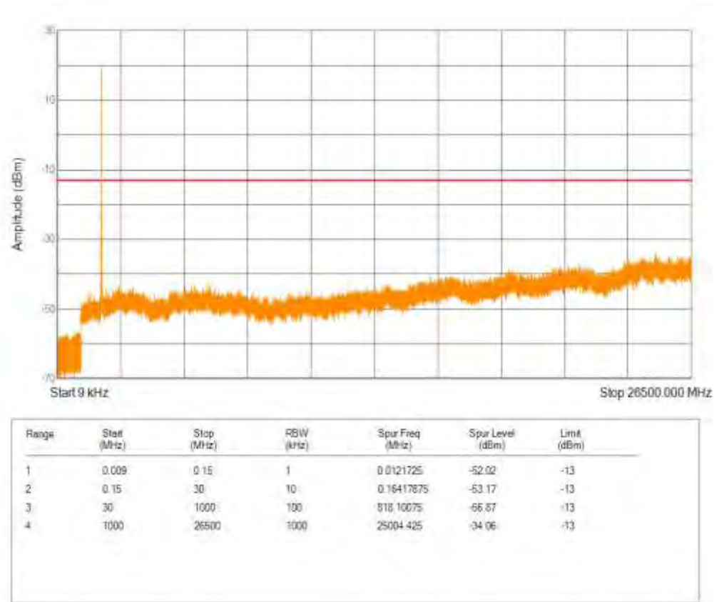
Band2 QAM16 BW=10MHz Channel=19150 RB Size=50 Position=#0
