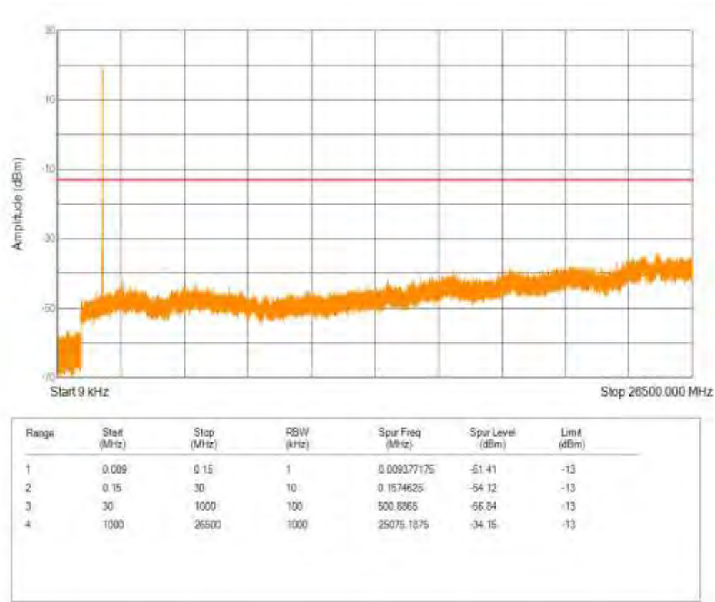
Band2 QAM16 BW=15MHz Channel=18675 RB Size=75 Position=#0
