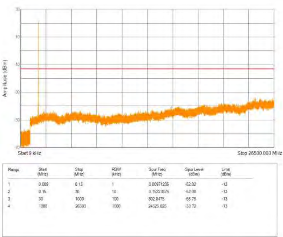
Band2 QPSK BW=1.4MHz Channel=18607 RB Size=6 Position=#0
