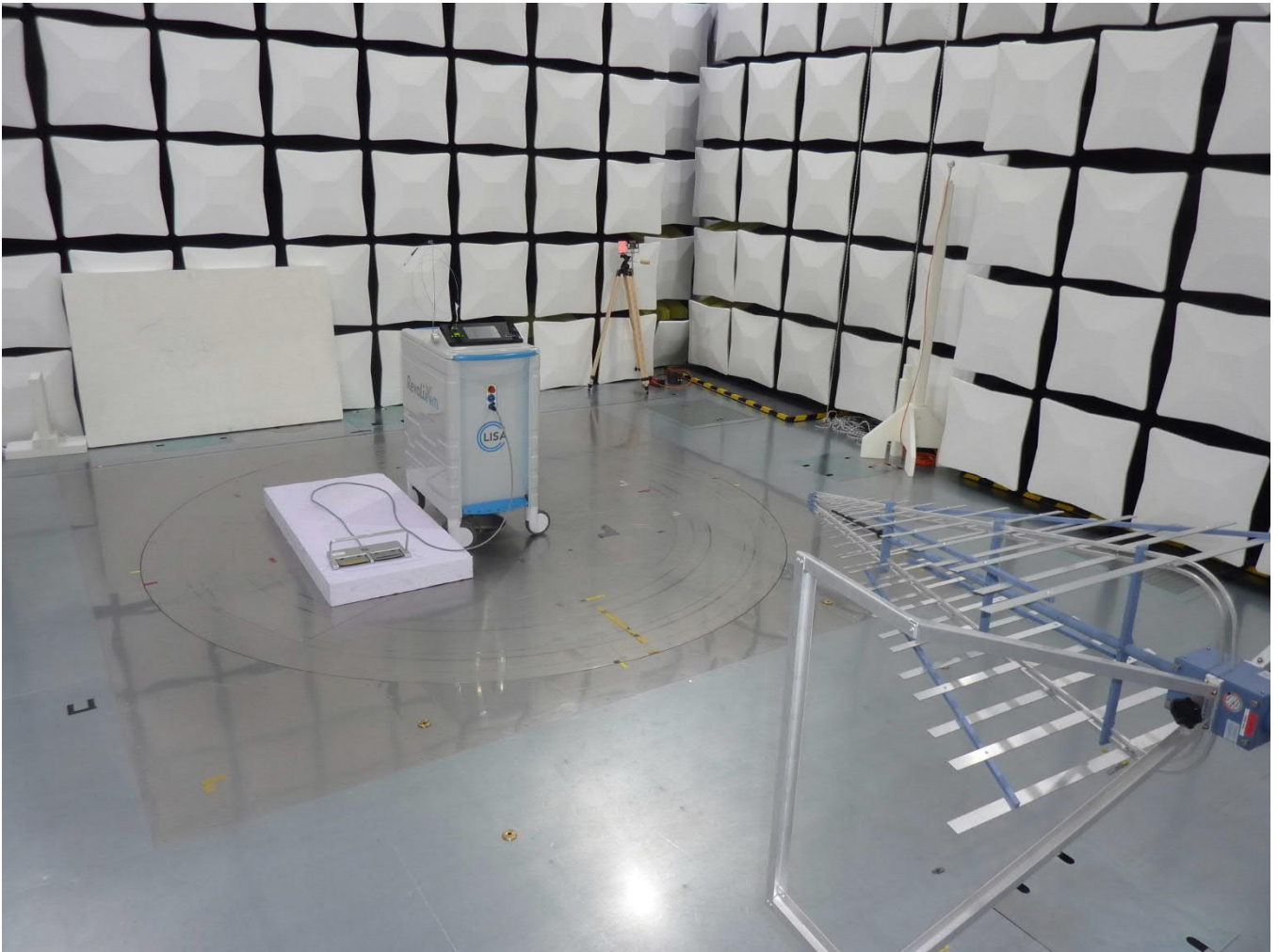
220394_03: Test setup radiated emission SAC 30 MHz - 1GHz
