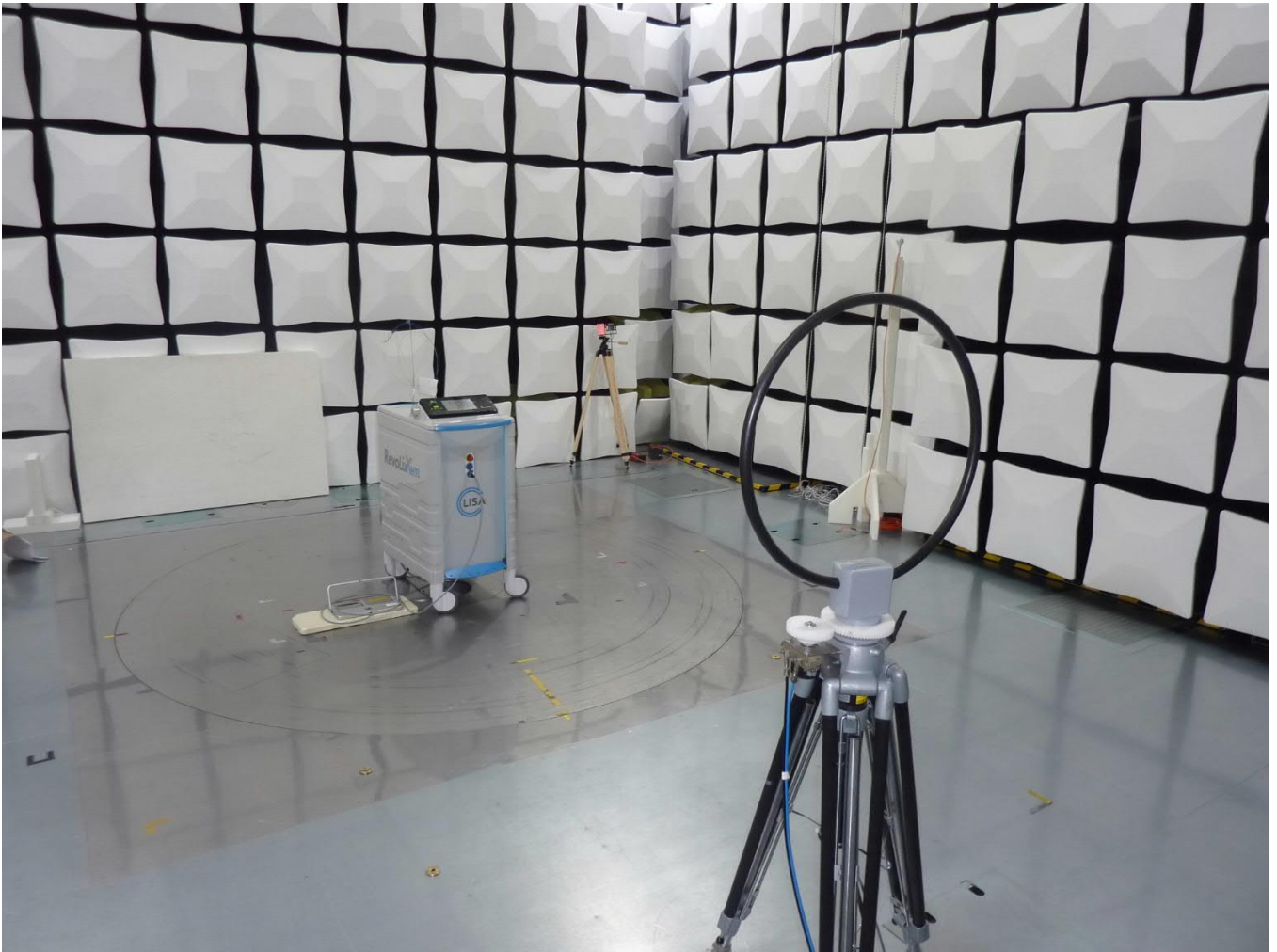
220394_01: Test setup preliminary measurement 9 kHz – 30 MHz
