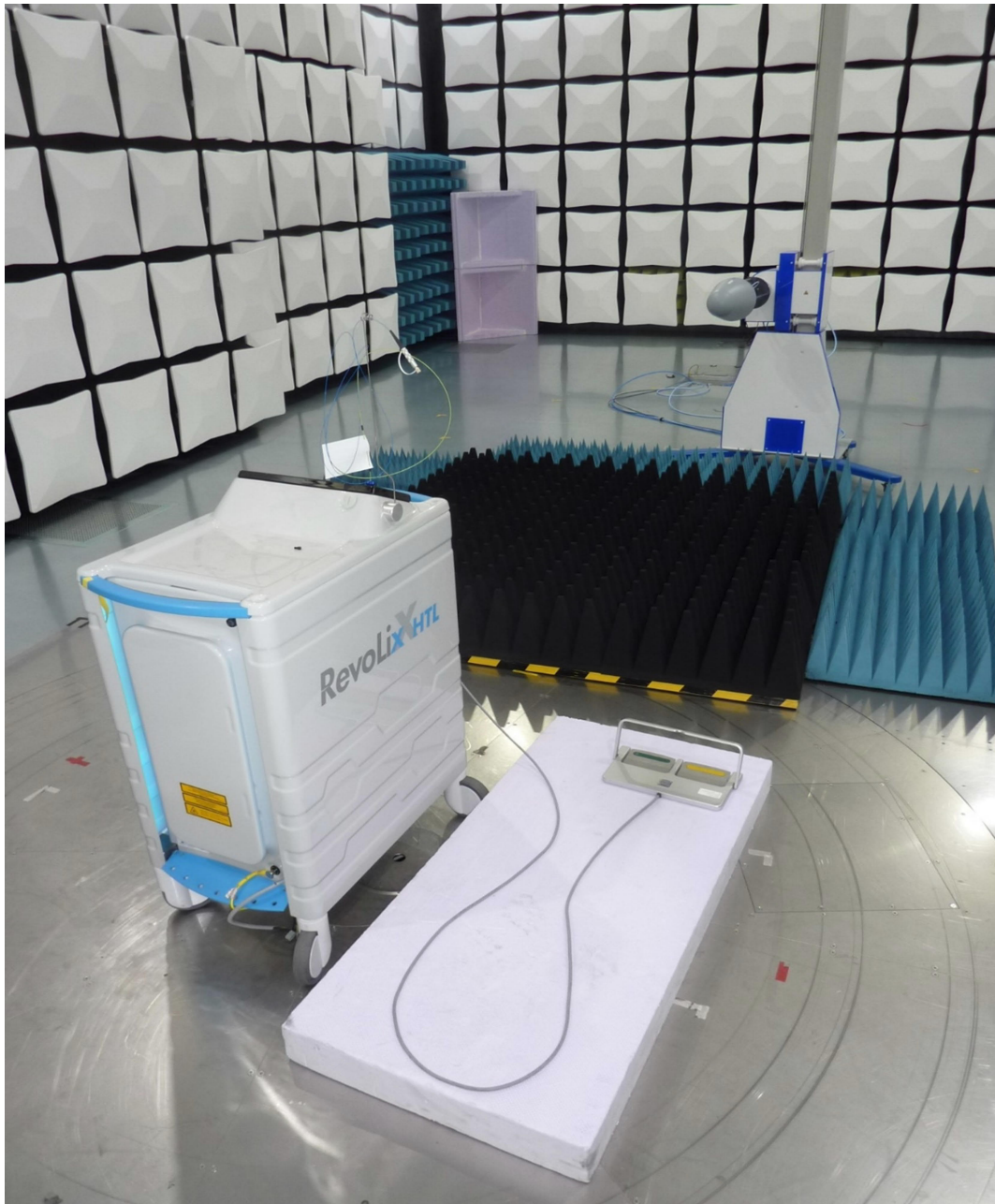
220394_04 Test setup radiated emission SAC 1 GHz – 12 GHz
