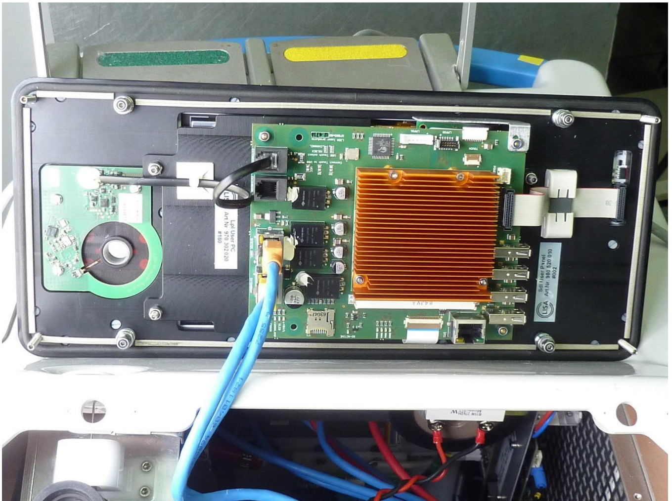
220394_EUT30: Control panel connectors
