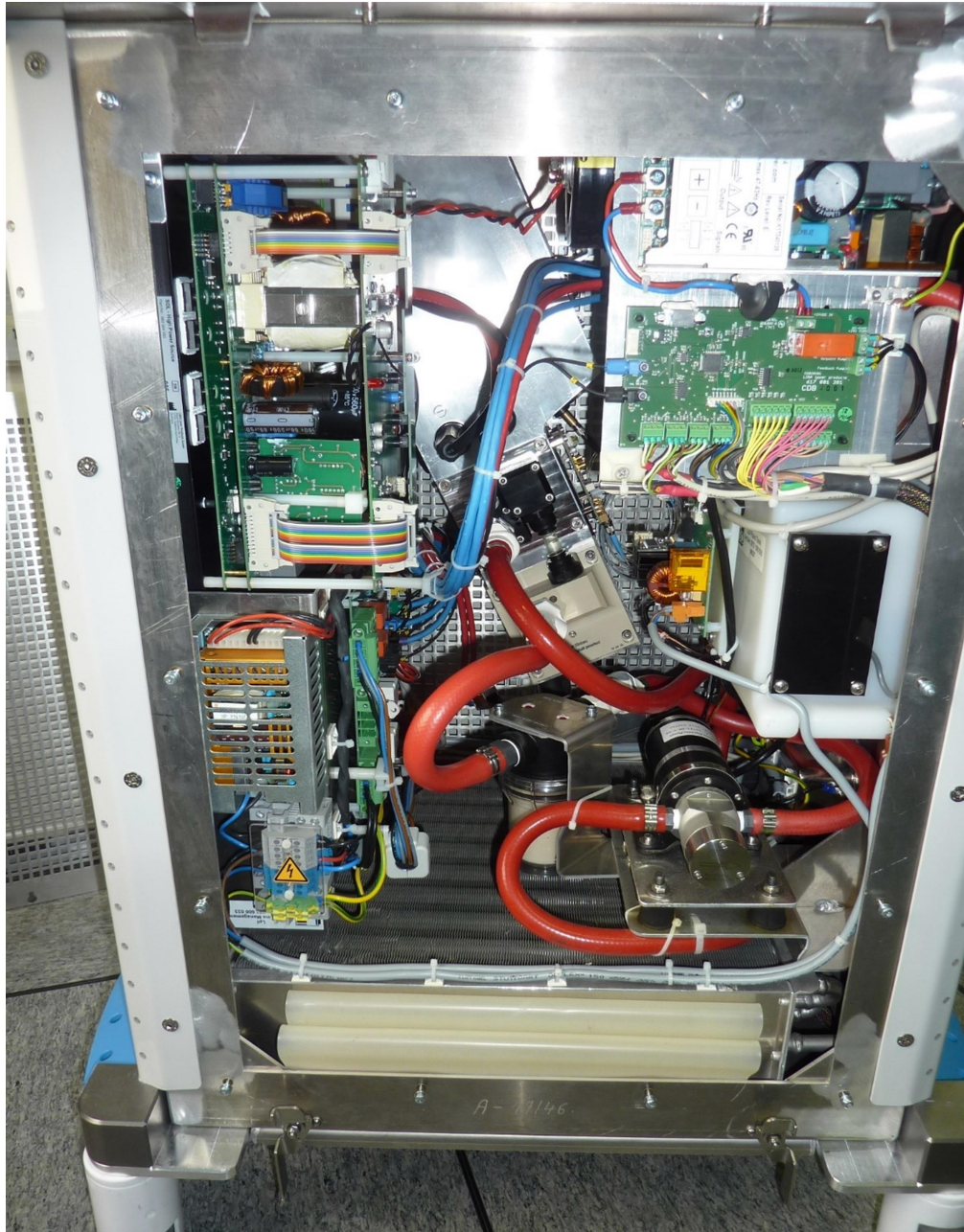
220394_EUT34: Inside view 3
