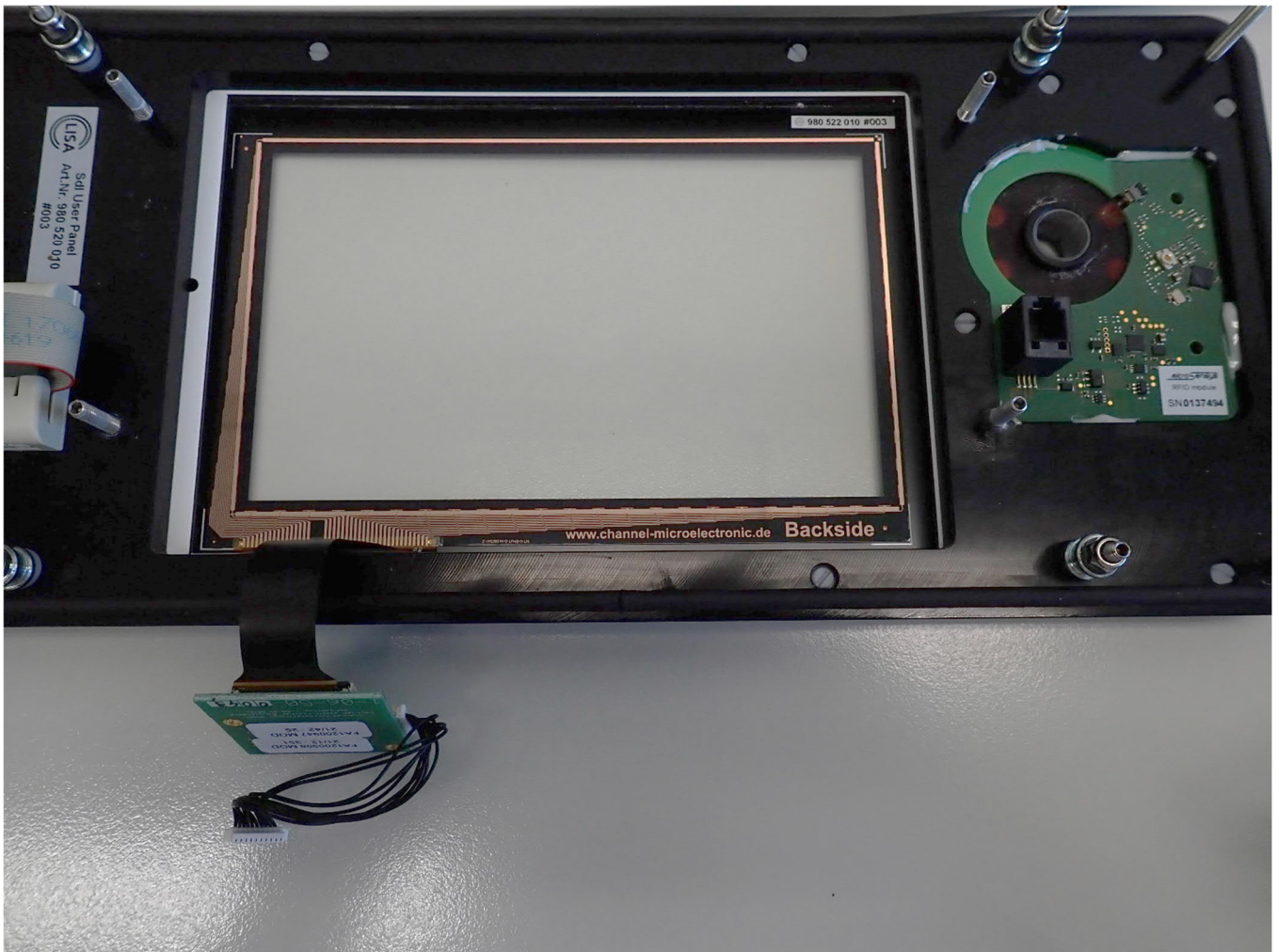
220394_EUT29*: Display panel view 3
