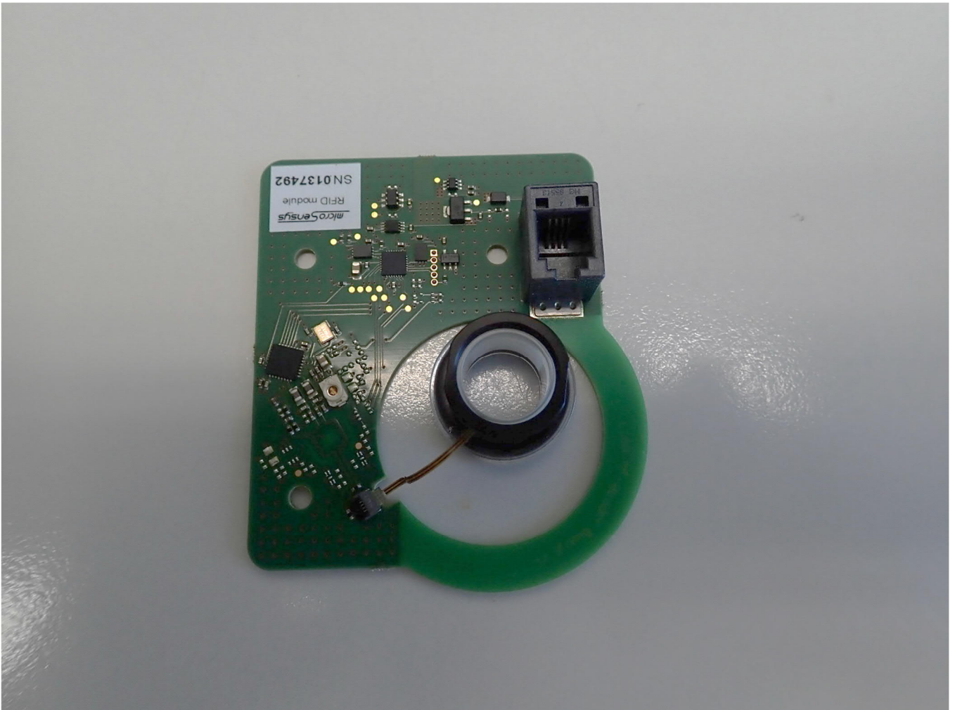
220394_EUT25: RFID reader PCB view 2
