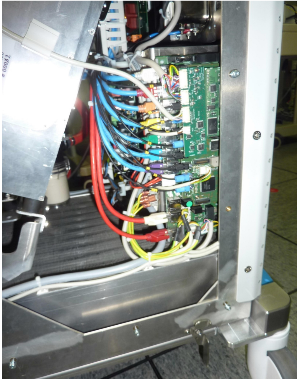
220394_EUT30: Inside view 6
