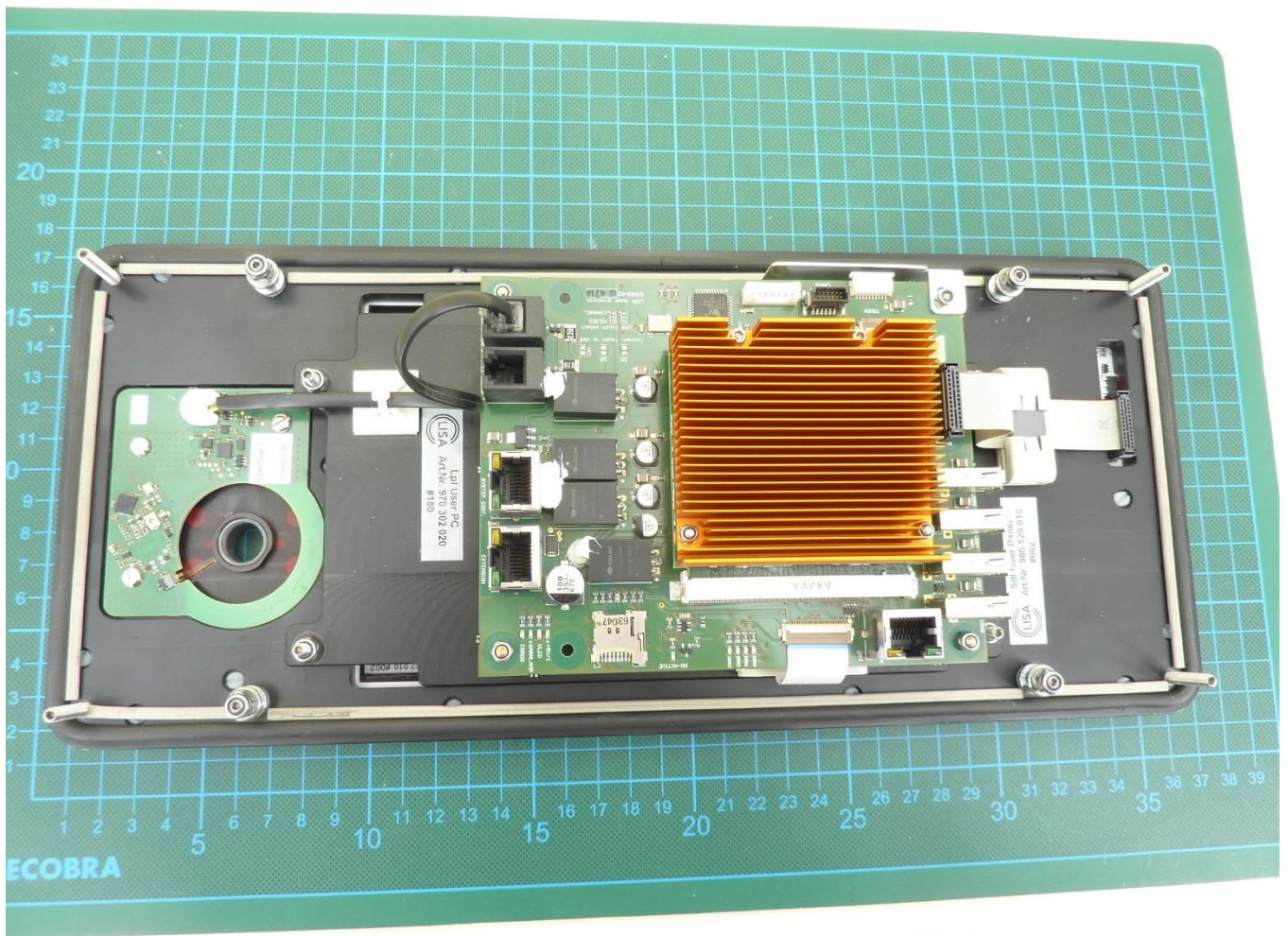
220394_EUT21: Control panel with RFID reader rear view
