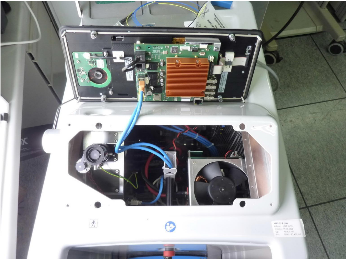
220394_EUT32: Inside view 1
