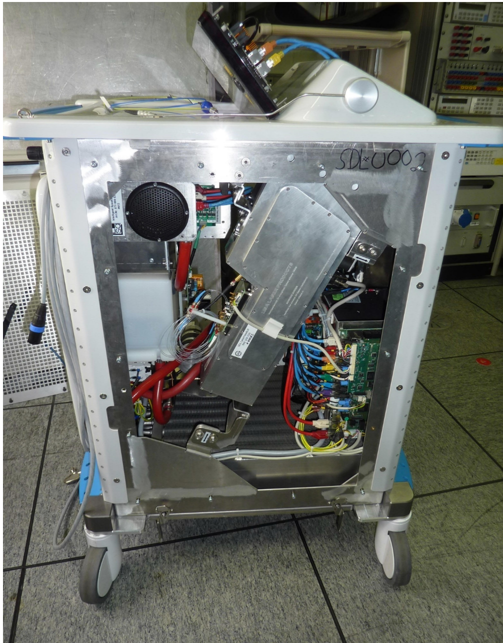
220394_EUT36: Inside view 5
