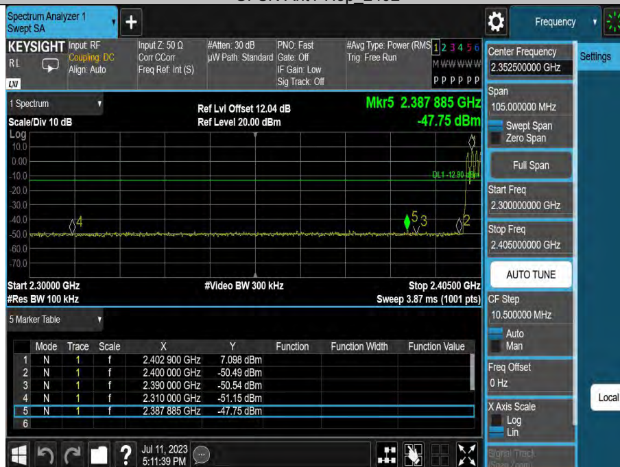
GFSK-Ant2-Hop_2402
