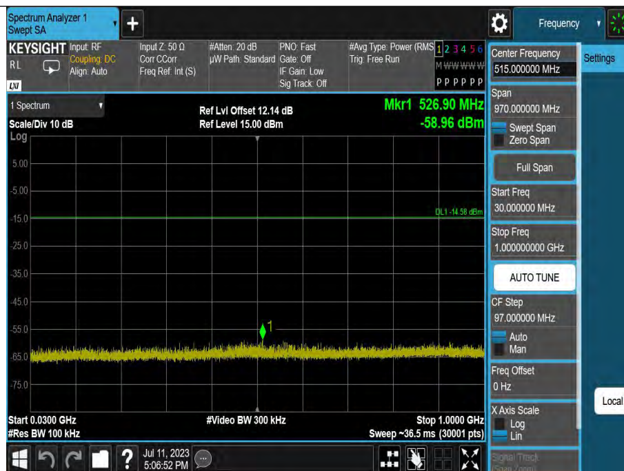
GFSK-Ant2-2480-30~1000
