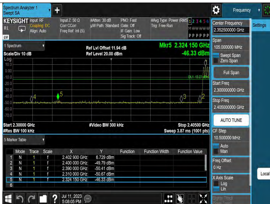
GFSK-Ant1-Hop_2402
