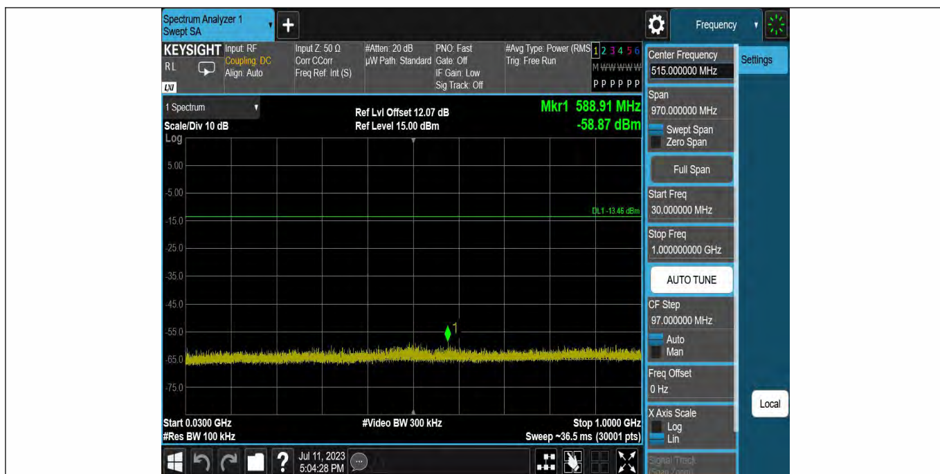
GFSK-Ant2-2441-30~1000
