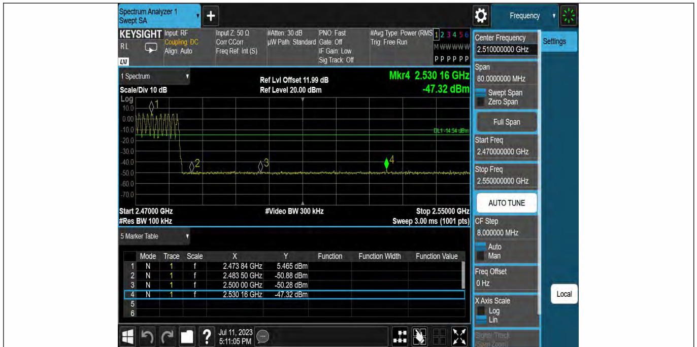
GFSK-Ant1-Hop_2480
