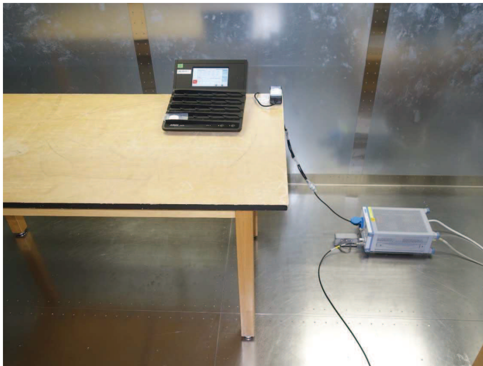
Photograph 6: Set-up for AC Power Line Conducted Emission of Transmitter, Front View
