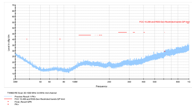
Figure 7.6-25: Radiated spurious emissions 30-1000 MHz
