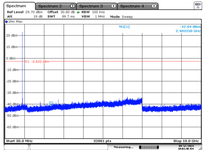
Figure 7.10-15: Conducted spurious emissions on 3.6 MHz Mid channel
