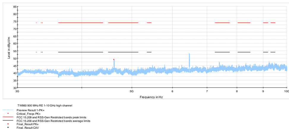
Figure 7.10-32: Radiated spurious emissions on 3-10 GHz High channel TW-860
