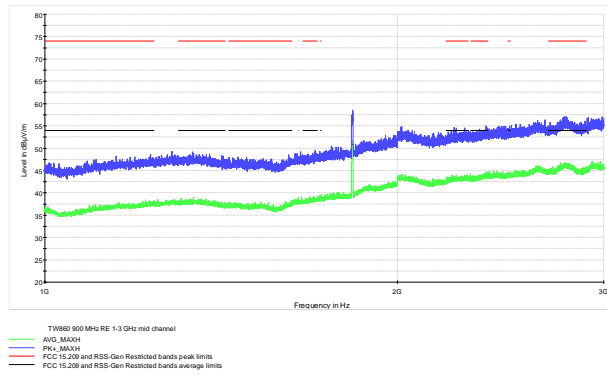
Figure 7.10-28: Radiated spurious emissions on 1-3 GHz Mid channel TW-860
