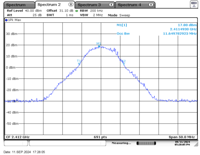
Figure 7.4-8: 99% bandwidth 10 MHz Sample Plot
