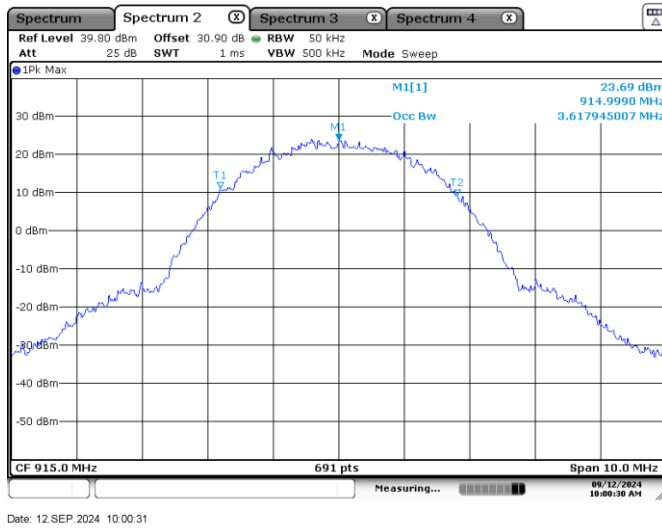
Figure 7.8-7: 99% bandwidth 3.6 MHz Sample Plot
