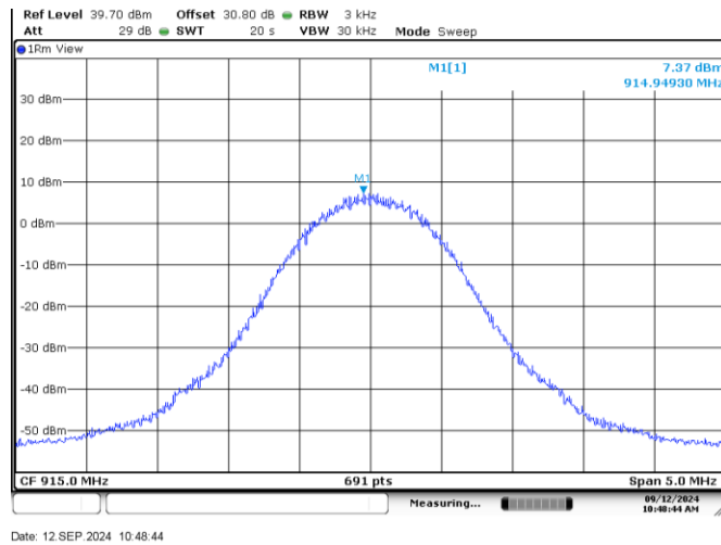
Figure 7.11-1: Example PSD 1.3 MHz
