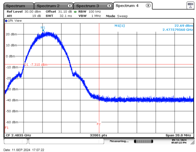
Figure 7.6-4: Band edge spurious emissions at 2483.5 MHz 3.6 MHz
