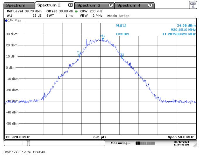
Figure 7.8-8: 99% bandwidth 10 MHz Sample Plot
