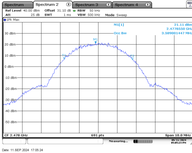
Figure 7.4-7: 99% bandwidth 3.6 MHz Sample Plot
