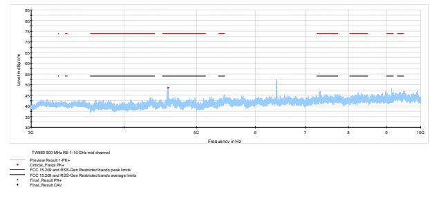
Figure 7.10-31: Radiated spurious emissions on emissions 3-10 GHz Mid channel TW860
