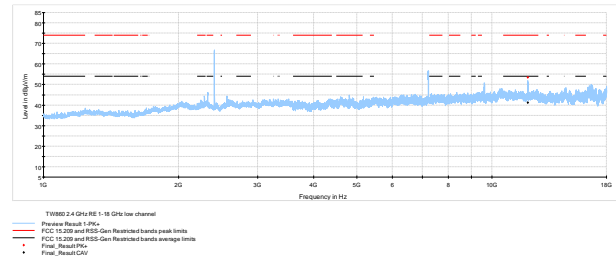
Figure 7.6-27: Radiated spurious emissions on emissions 1-18 GHz
