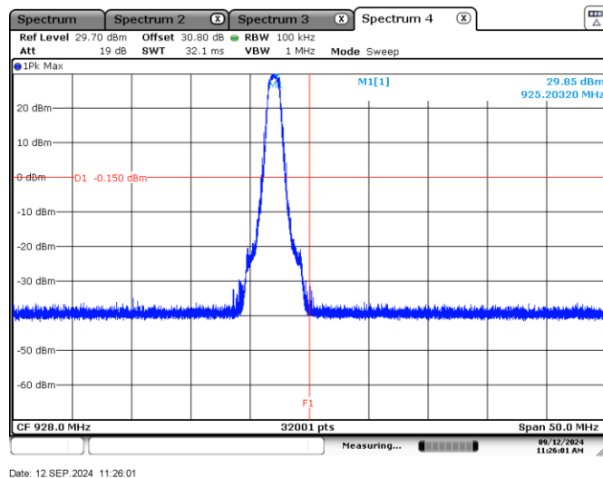
Figure 7.10-2: Band edge spurious emissions at 928 MHz 1.3 MHz
