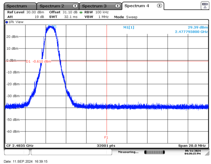
Figure 7.6-2: Band edge spurious emissions at 2483.5 MHz 1.2 MHz
