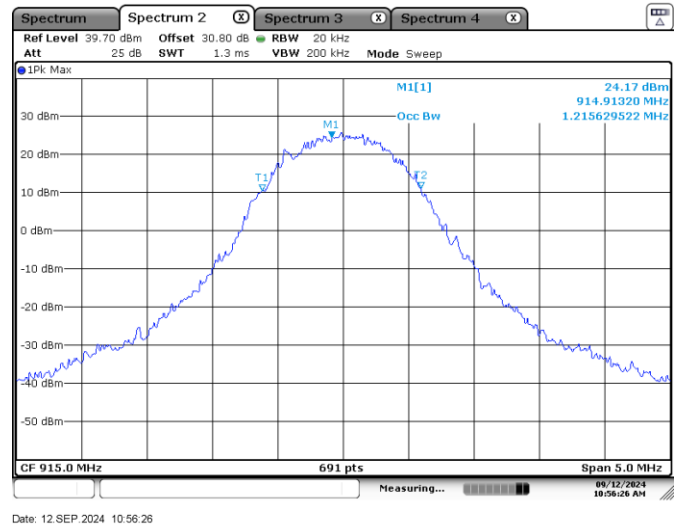
Figure 7.8-6: 99% bandwidth 1.3 MHz Sample Plot
