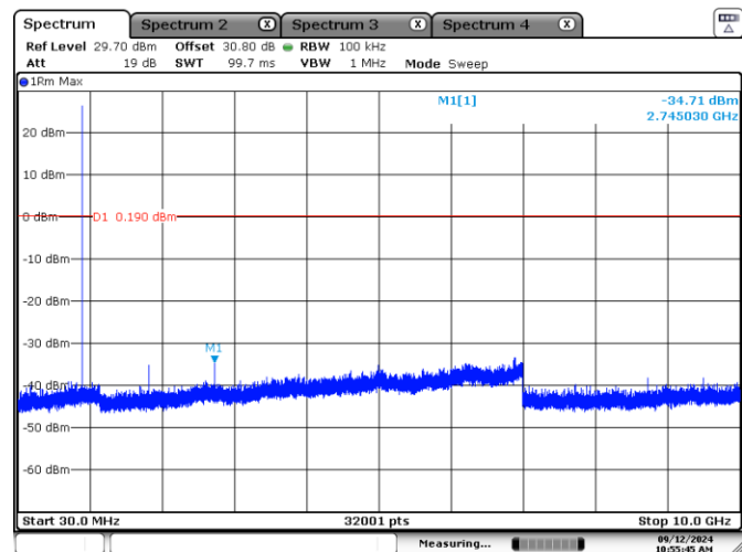
Figure 7.10-12: Conducted spurious emissions on 1.3 MHz Mid channel
