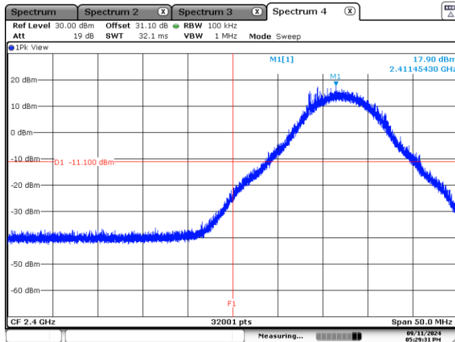
Figure 7.6-5: Band edge spurious emissions at 2400 MHz 10 MHz
