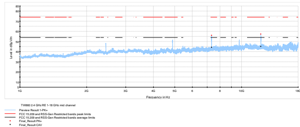
Figure 7.6-28: Radiated spurious emissions on 1-18 GHz Mid channel TW-860
