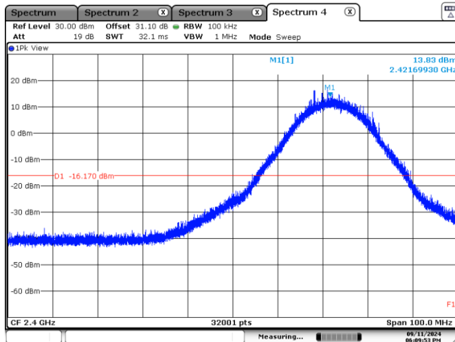
Figure 7.6-7: Band edge spurious emissions at 2400 MHz 20 MHz
