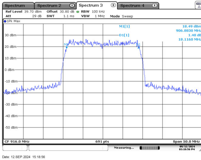
Figure 7.8-5: 6 dB bandwidth HDR 20 MHz Sample Plot
