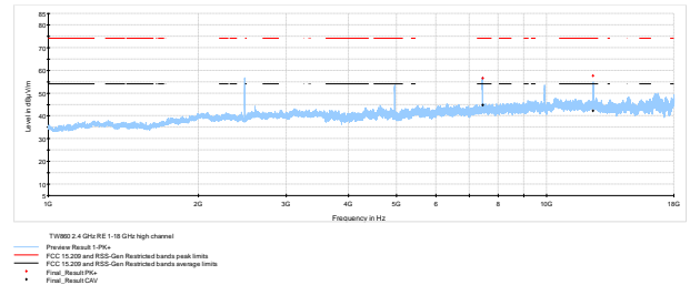
Figure 7.6-29: Radiated spurious emissions 1-18 GHz High channel TW-860
