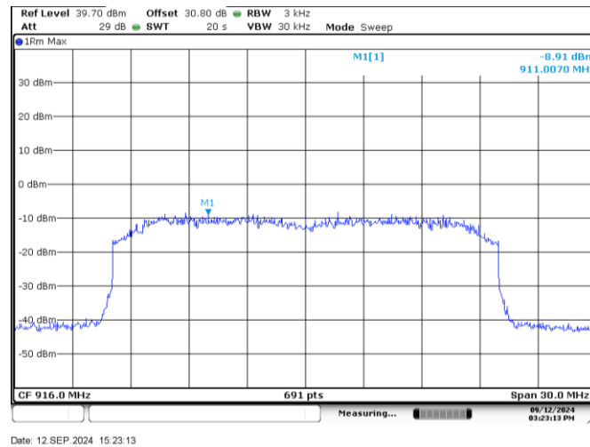
Figure 7.11-5: Example PSD HDR 20 MHz
