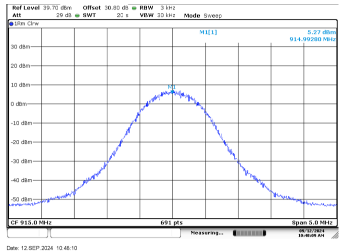
Figure 7.11-2: Example PSD 3.6 MHz
