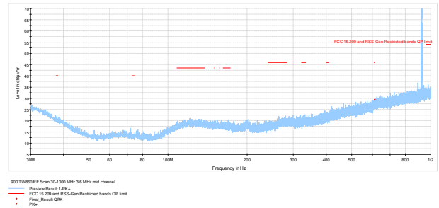
Figure 7.10-25: Radiated spurious emissions 30-1000 MHz Mid channel TW-860
