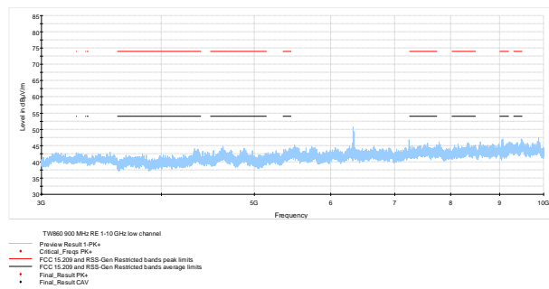
Figure 7.10-30: Radiated spurious emissions 3-10 GHz Low channel TW-860
