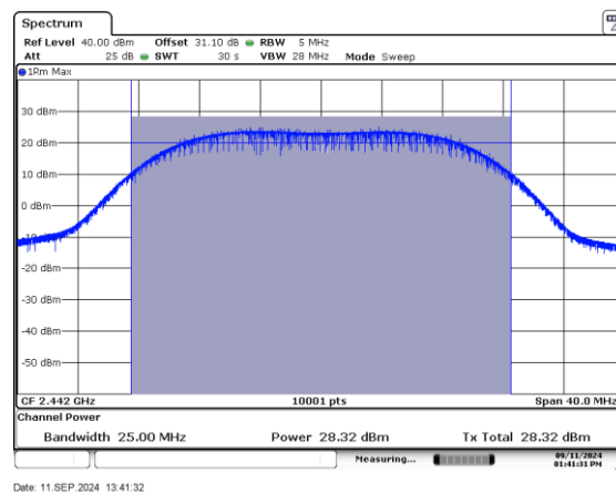
Figure 7.5-5: Conducted Output Power HDR 20 MHz sample plot
