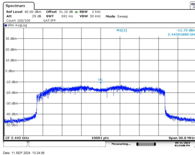
Figure 7.7-5: Example PSD HDR 20 MHz
