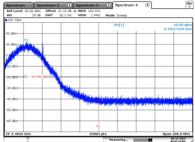
Figure 7.6-8: Band edge spurious emissions at 2483.5 MHz 20 MHz
