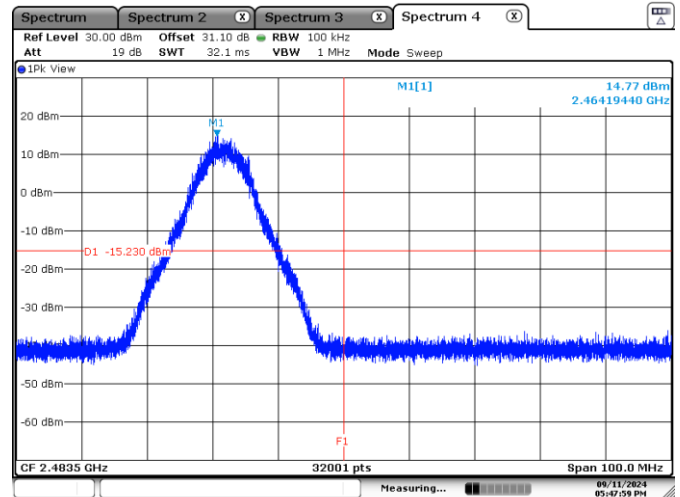
Figure 7.6-6: Band edge spurious emissions at 2483.5 MHz 10 MHz
