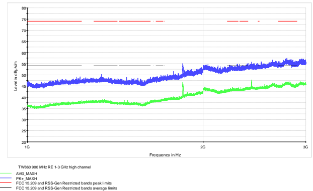
Figure 7.10-29: Radiated spurious emissions 1-3 GHz High channel TW-860
