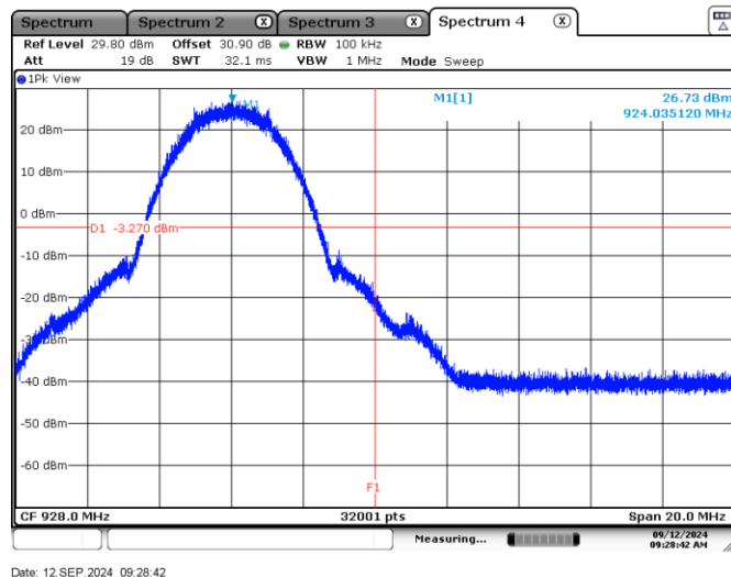
Figure 7.10-4: Band edge spurious emissions at 928 MHz 3.6MHz
