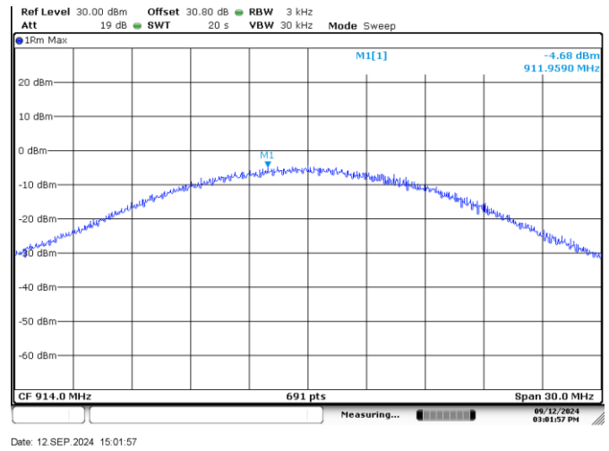
Figure 7.11-4: Example PSD 20 MHz
