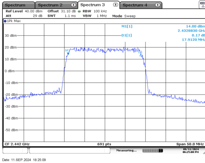
Figure 7.4-5: 6 dB bandwidth HDR 20 MHz Sample Plot
