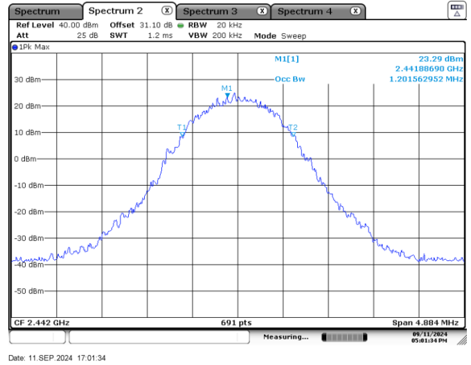
Figure 7.4-6: 99% bandwidth 1.2 MHz Sample Plot
