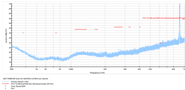
Figure 7.10-24: Radiated spurious emissions on 30-1000 MHz Low channel TW-860
