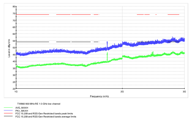
Figure 7.10-27: Radiated spurious emissions on emissions 1-3 GHz Low channel TW860
