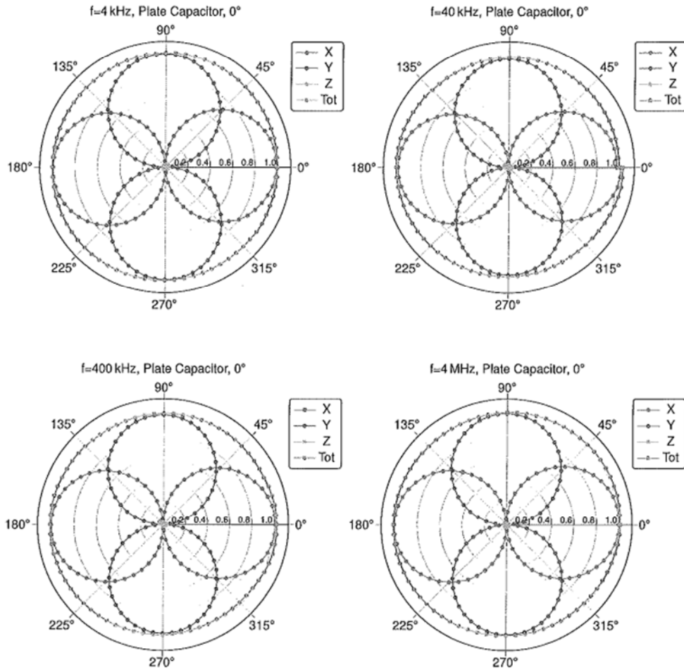
E-Field Receiving Pattern ( \phi ), \theta = 0^\circ
