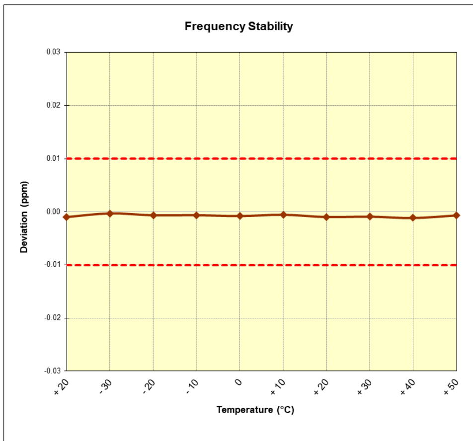
Figure 7-3. Frequency Stability Plot
