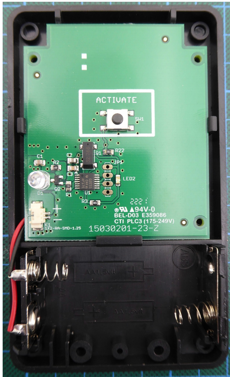
Transmitter Top view
