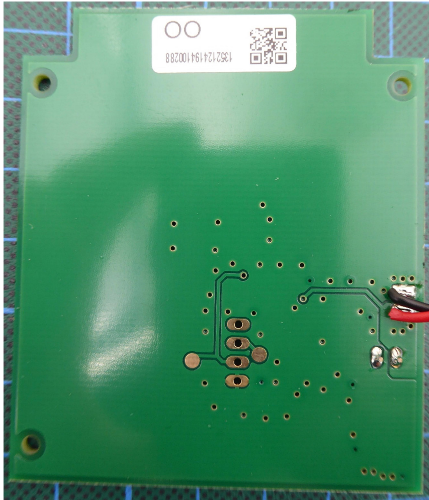
Transmitter bottom view
