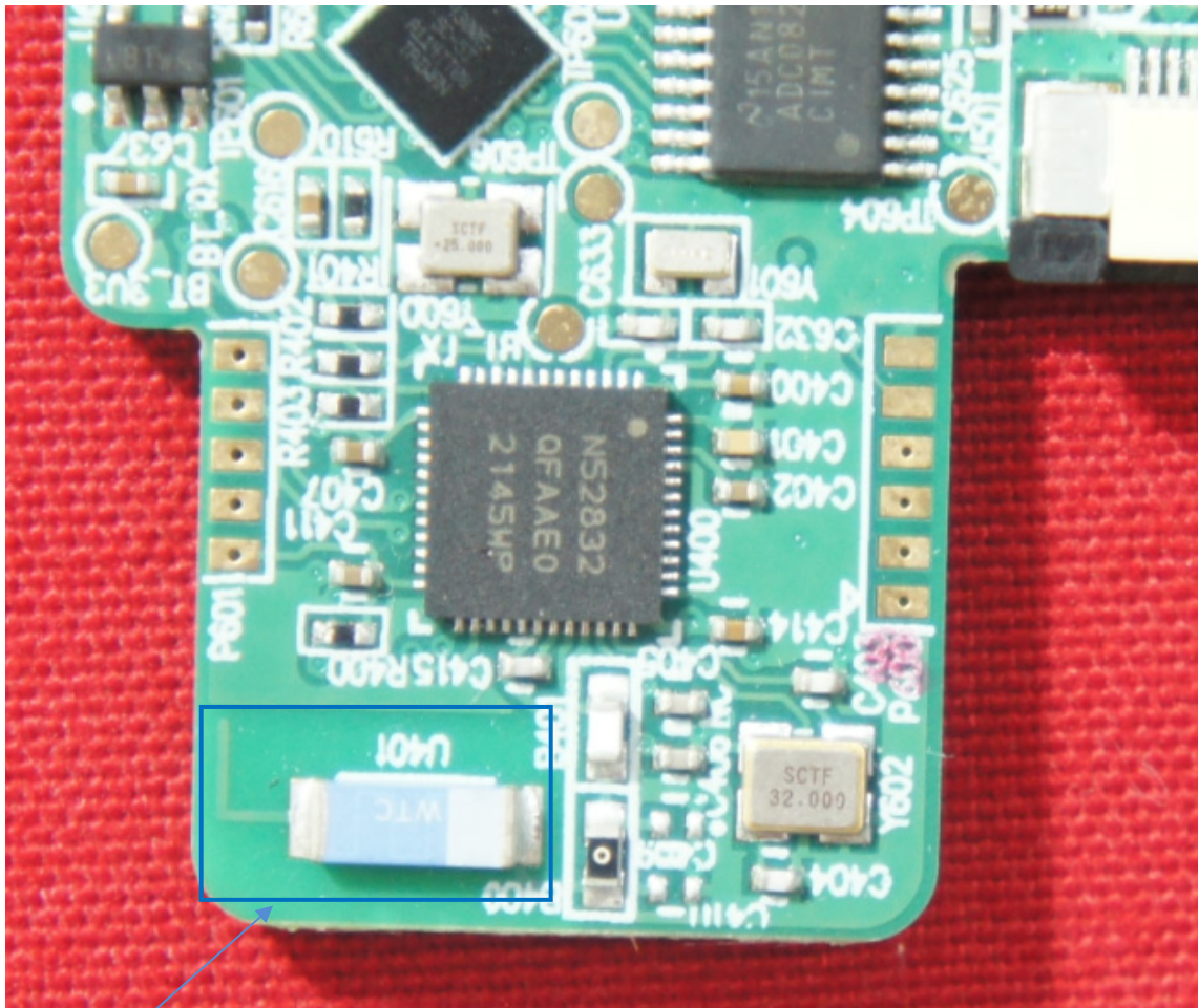
Bluetooth Antenna
