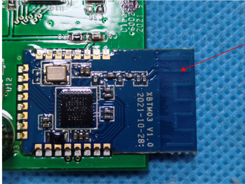
BTAntenna
