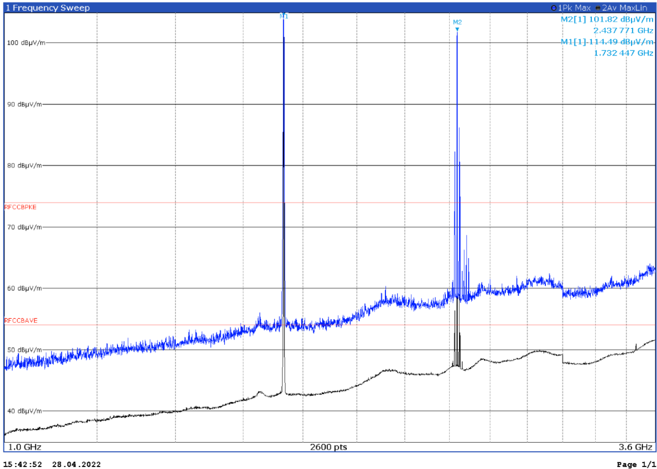
Figure 8.1-12: Radiated spurious emissions with LTE B4 at mid channel and WIFI at mid channel – antenna in vertical polarization
