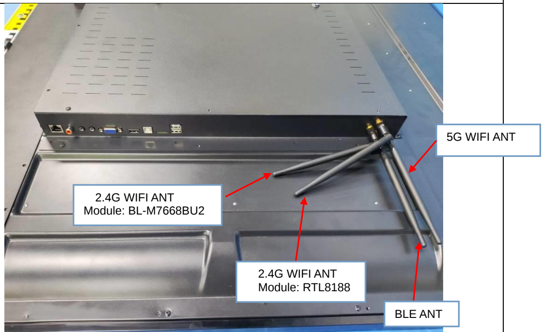
Antenna photo
