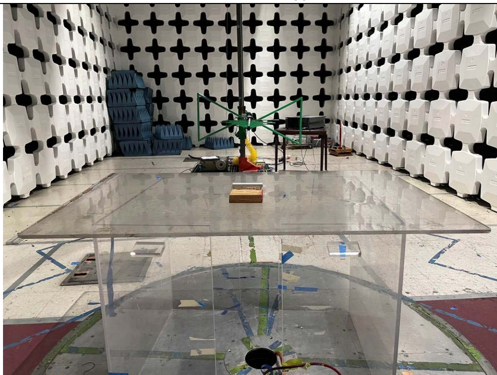
Radiated Emission Test below 30MHz Rear View
