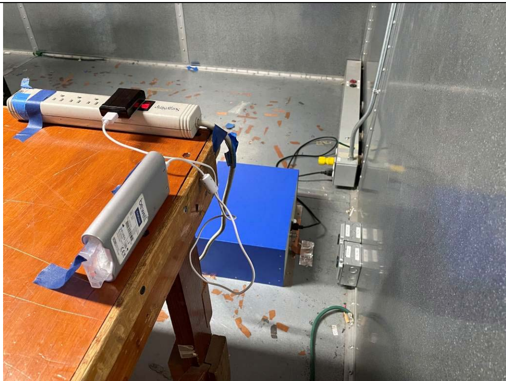
AC Line Conducted Emission Rear View
