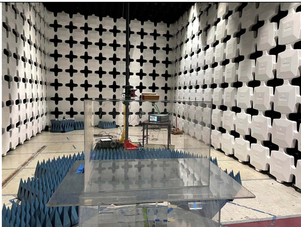
Radiated Emission Test above 1GHz Rear View
