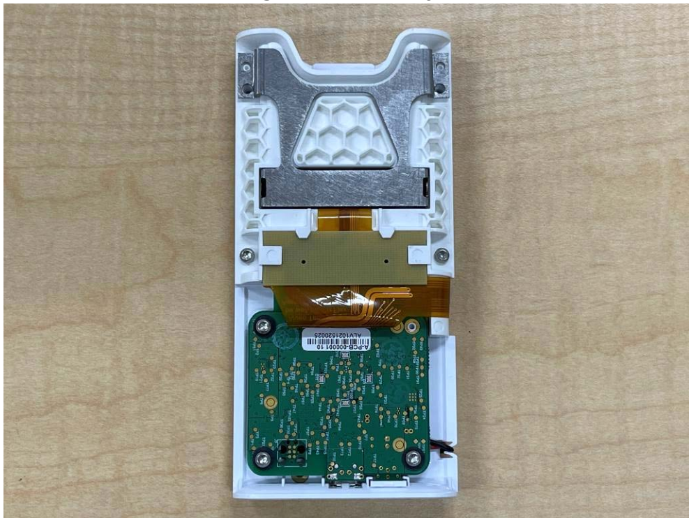
EUT Open the Enclosure View
