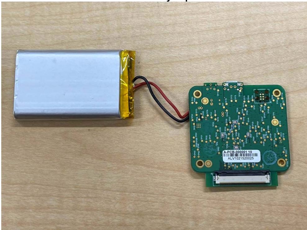
PCB With Battery Bottom View
