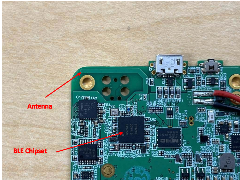
Radio Module With Antenna View
