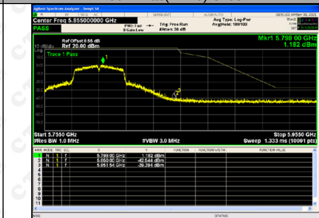
802.11ac(VH40)-5795
