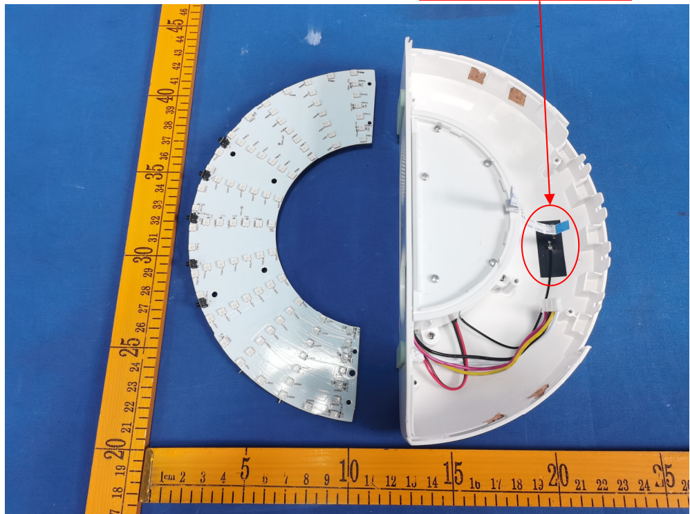
BT/BLE antenna
