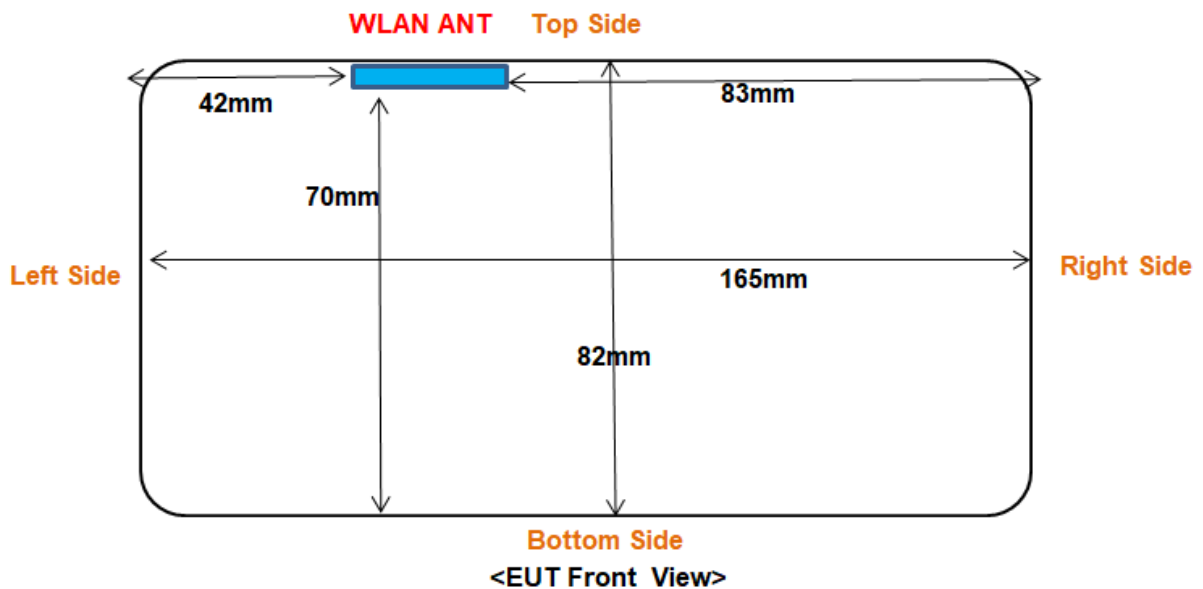
Fig 7.1 Block Diagram for EUT Antenna Position
