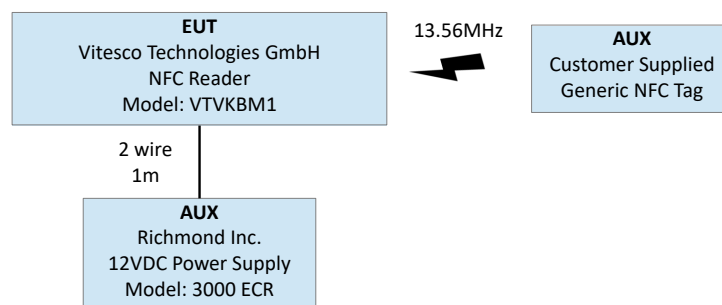
Figure 2: EUT Test Configuration Diagram.
