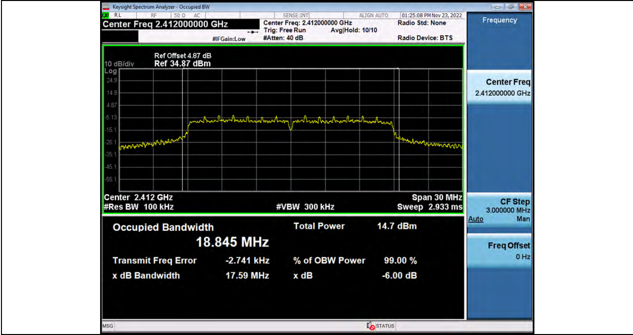
-6dB_Bandwidth_2_4GWiFi_802_11n(HT20)_2412
