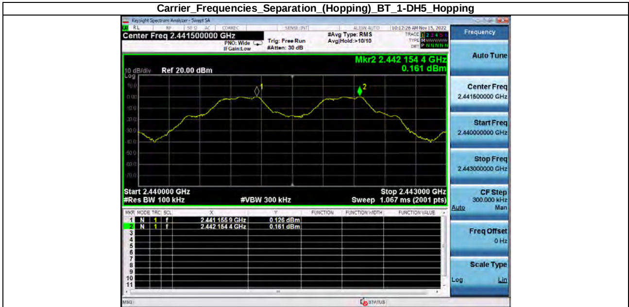
Carrier_Frequencies_Separation_(Hopping)_BT_1-DH5_Hopping
