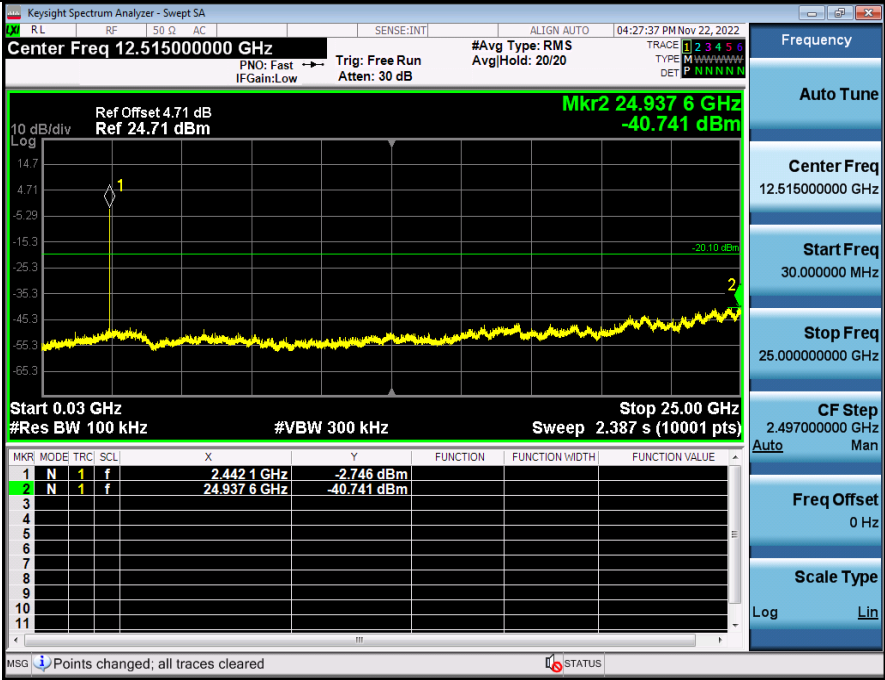
2_Spurious_Emissions_BT_3-DH5_2441
