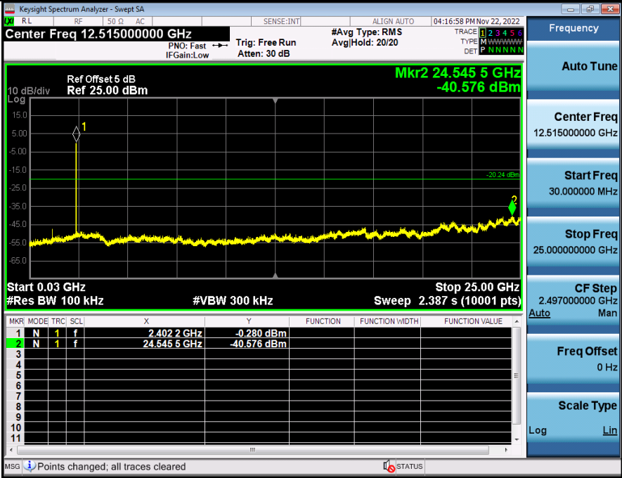
2_Spurious_Emissions_BT_2-DH5_2402
