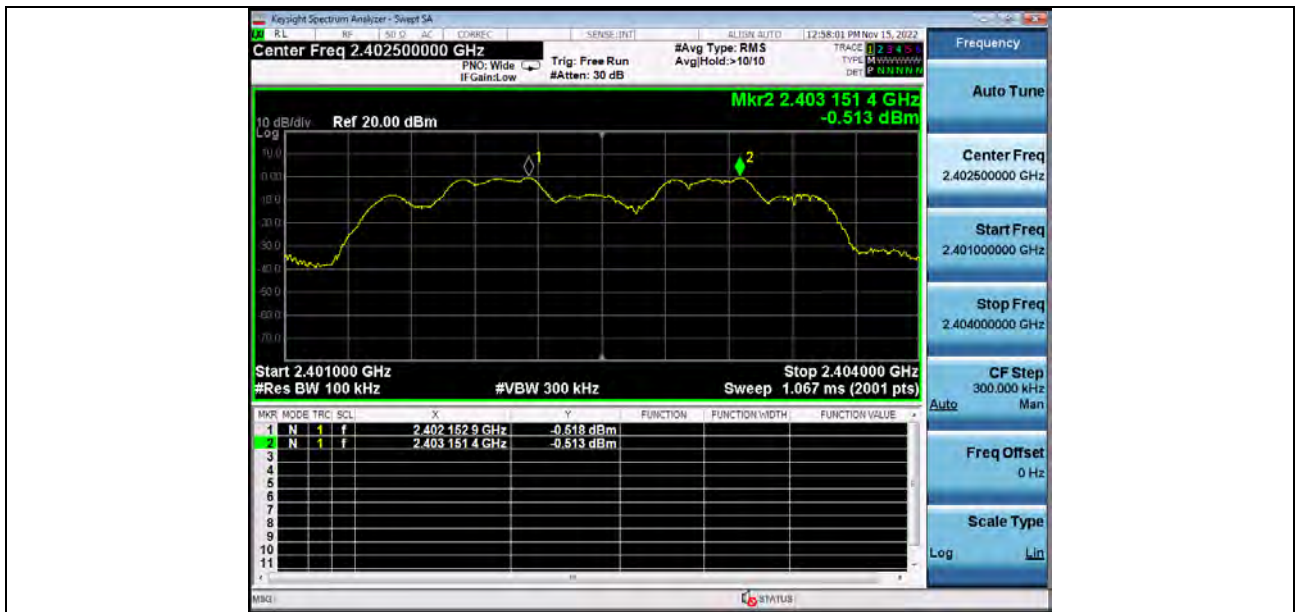
Carrier_Frequencies_Separation_(Hopping)_BT_3-DH5_Hopping
