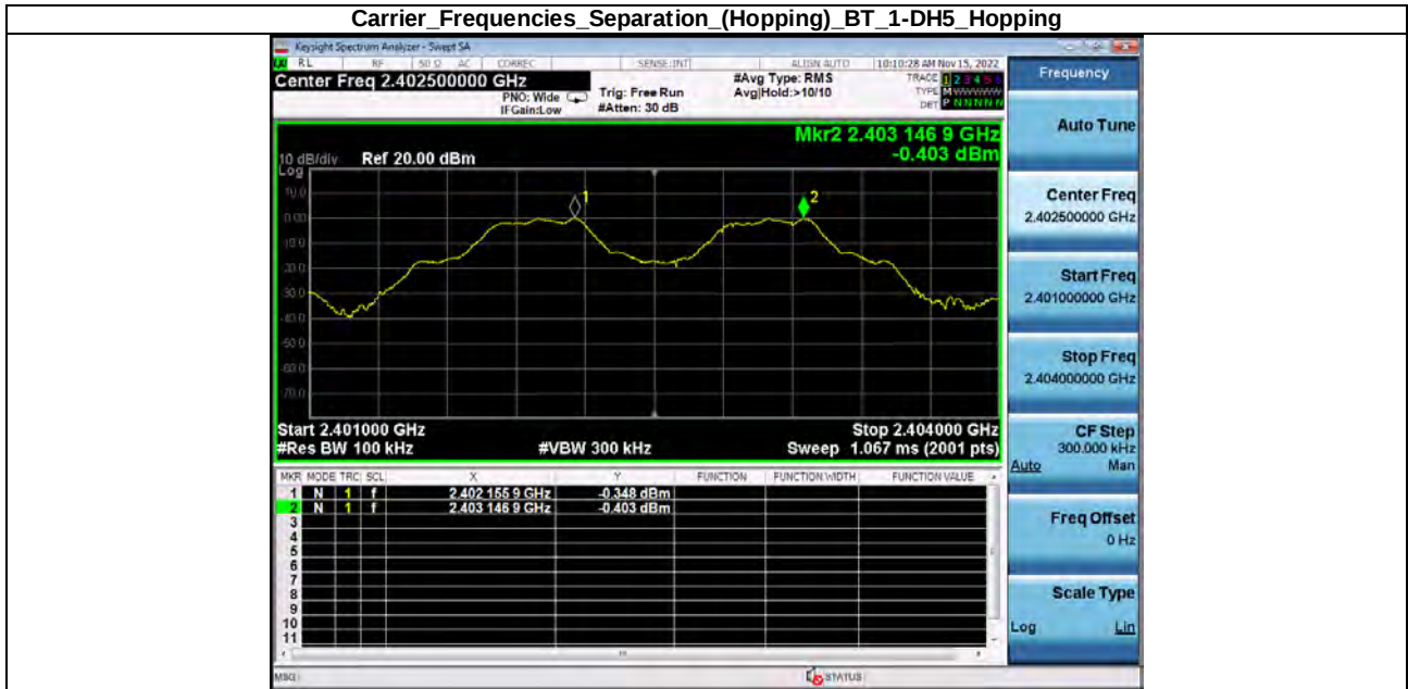
Carrier_Frequencies_Separation_(Hopping)_BT_1-DH5_Hopping
