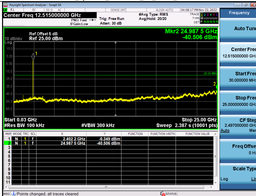
2 Spurious Emissions BT 1-DH5 2402
