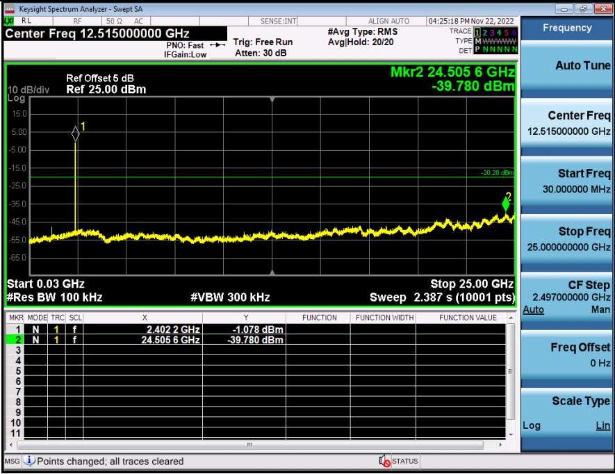
2_Spurious_Emissions_BT_3-DH5_2402
