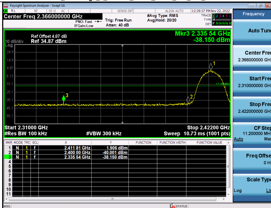
2 Bandedge 2 4GWiFi NVNT ANT1 802_11b 2412
