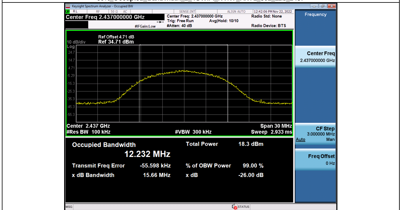
99% Occupied Bandwidth 2_4GWiFi_NVNT_ANT1_802_11b_2437
