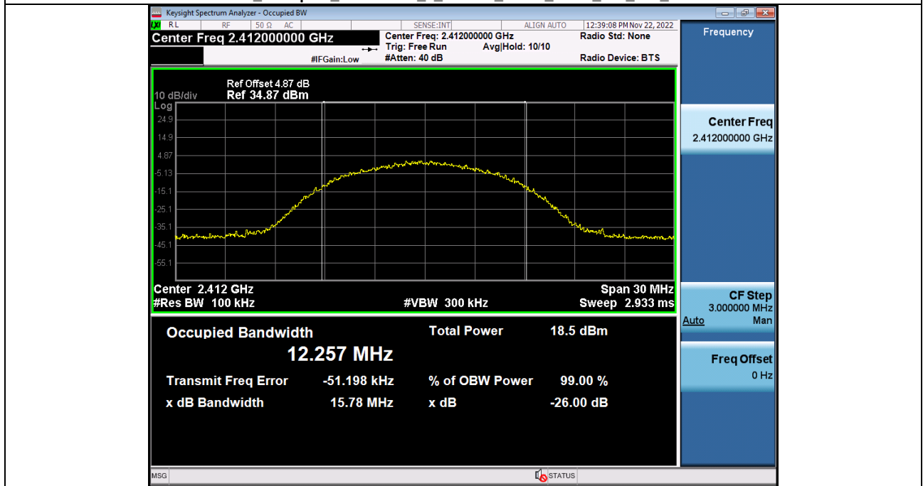
99% Occupied Bandwidth 2_4GWiFi_NVNT_ANT1_802_11b_2412
