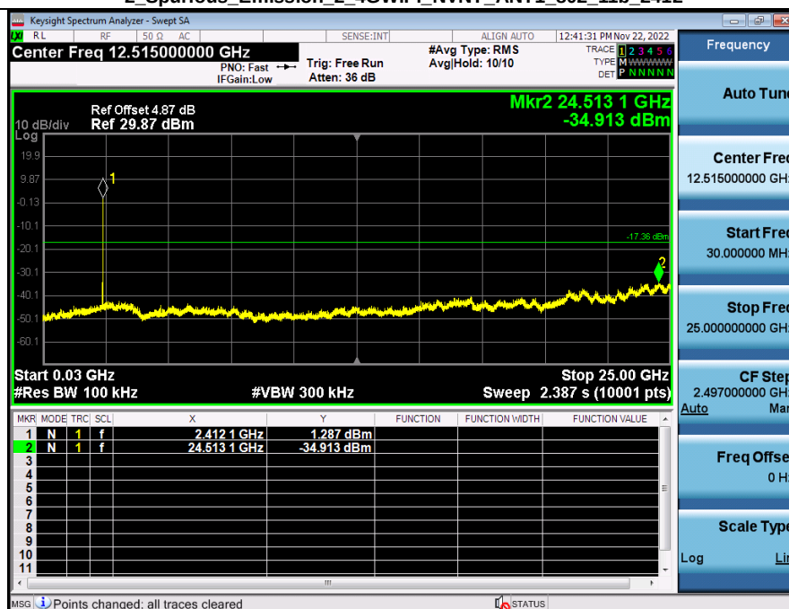
2. Spurious Emission 2_4GWiFi_NVNT_ANT1_802_11b_2412
