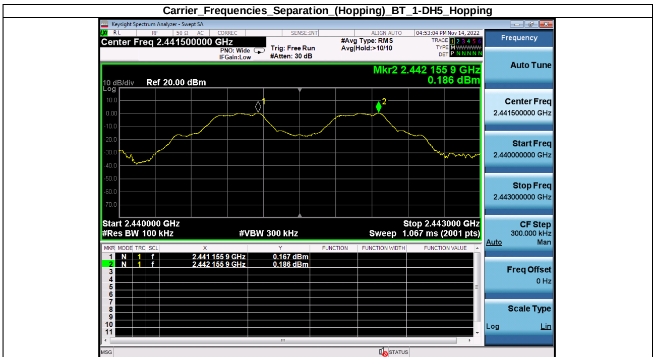
Carrier_Frequencies_Separation_(Hopping)_BT_1-DH5_Hopping
