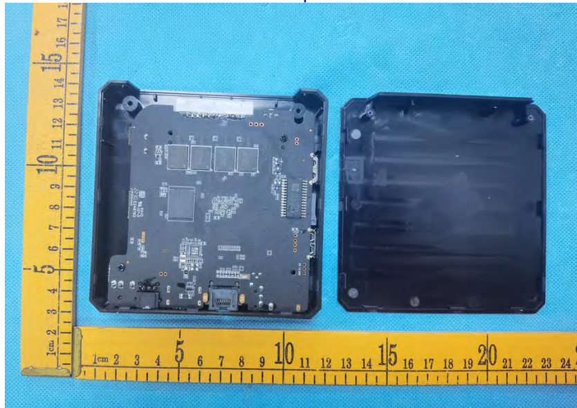
internal photos
