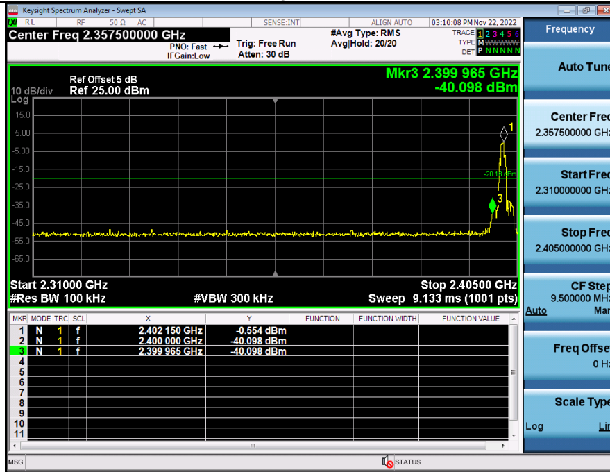
2_Bandedge_BT_2-DH5_2402
