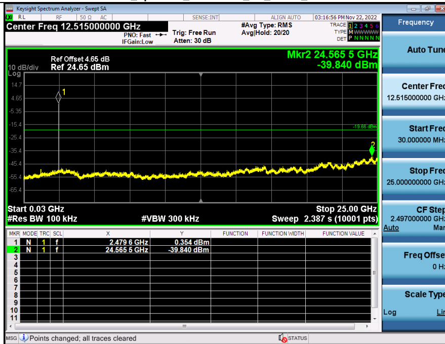
2_Spurious_Emissions_BT_2-DH5_2480
