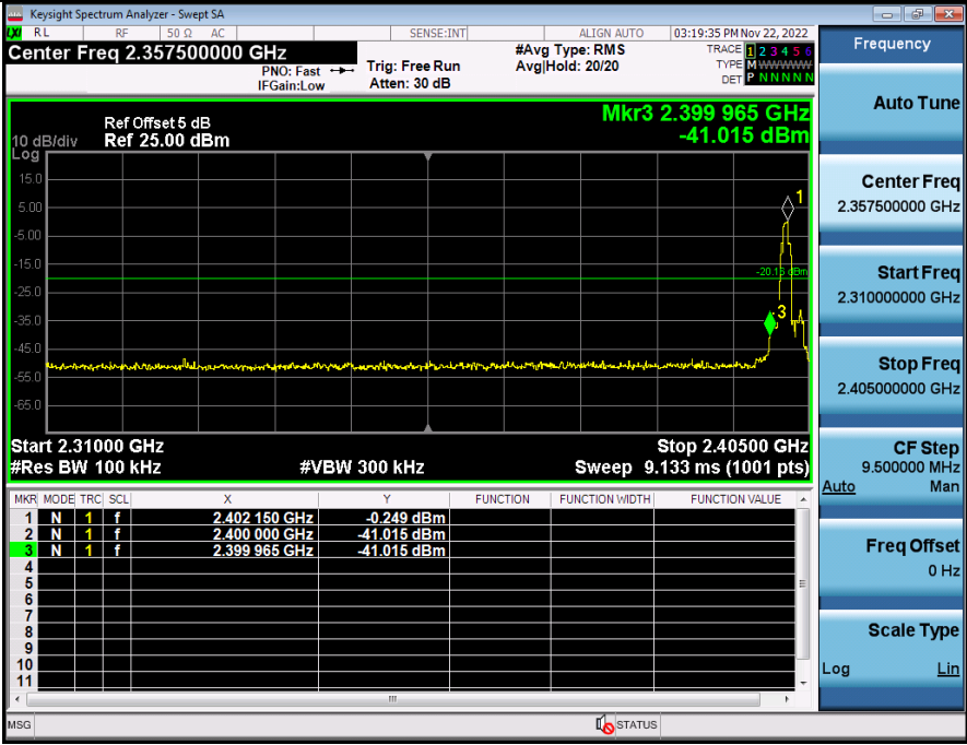
2_Bandedge_BT_3-DH5_2402
