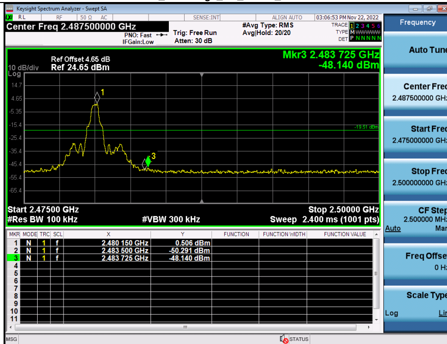
2_Bandedge_BT_1-DH5_2480
