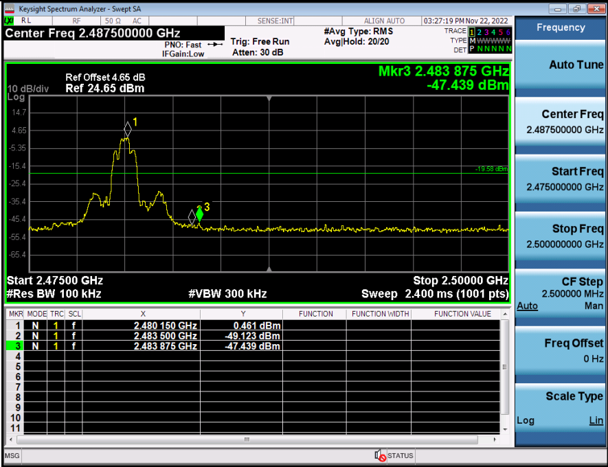
2_Bandedge_BT_3-DH5_2480
