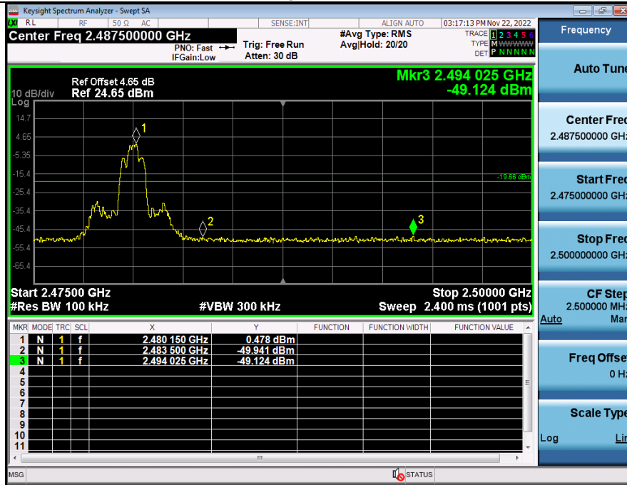
2_Bandedge_BT_2-DH5_2480
