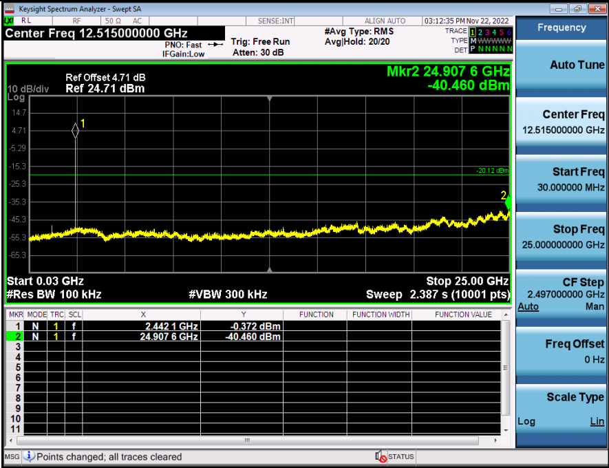
2_Spurious_Emissions_BT_2-DH5_2441
