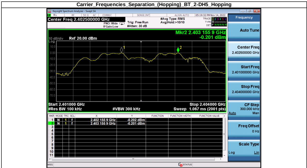
Carrier_Frequencies_Separation_(Hopping)_BT_2-DH5_Hopping
