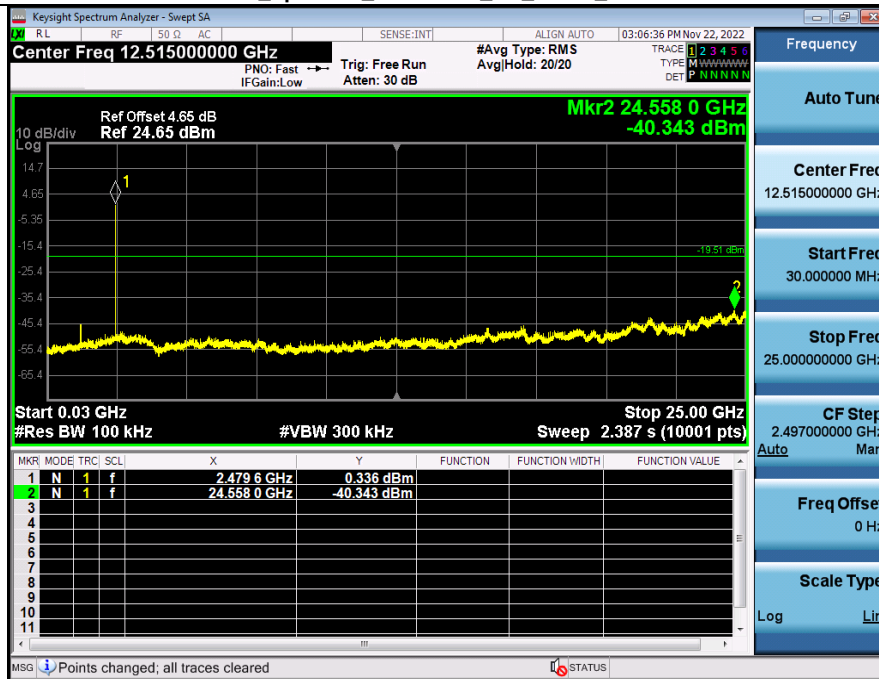
2_Spurious_Emissions_BT_1-DH5_2480
