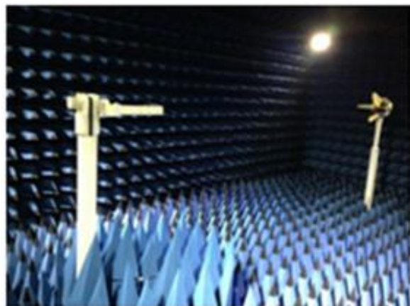
ETS darkroom
