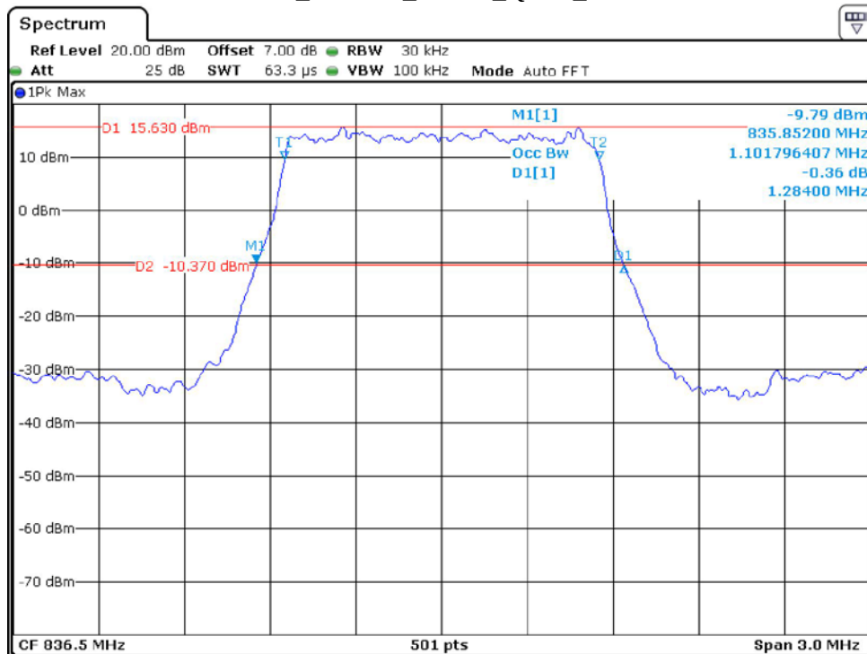
Band 5_1.4 MHz_Middle_QPSK_RB6#0
