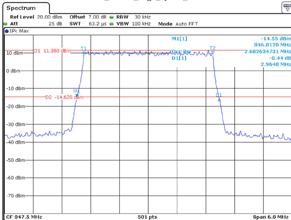
Band 5_3 MHz_High_QPSK_RB15#0
