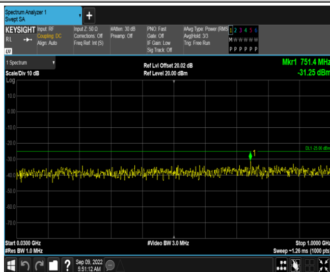
Band7-15MHz-QPSK-21375-1RB#0-Range1:30~1000MHz
