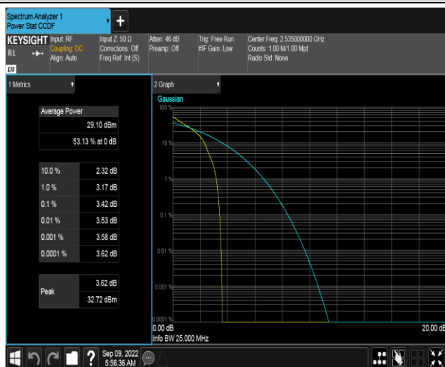
Band7-15MHz-QPSK-21100-1RB#0
