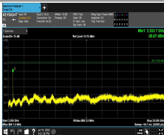
Band5-5MHz-16QAM-20625-1RB#0-Range3:2000~20000MHz
