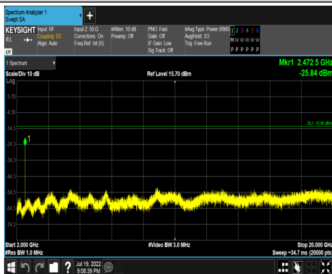
Band5-3MHz-16QAM-20415-1RB#0-Range3:2000~20000MHz
