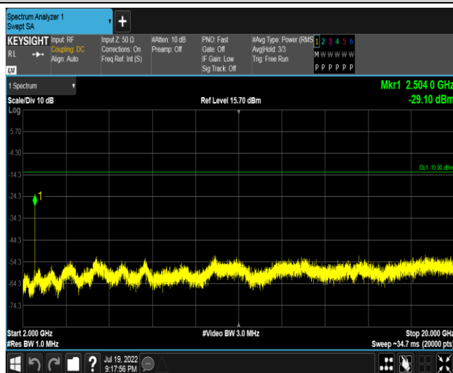
Band5-5MHz-QPSK-20525-1RB#0-Range3:2000~20000MHz
