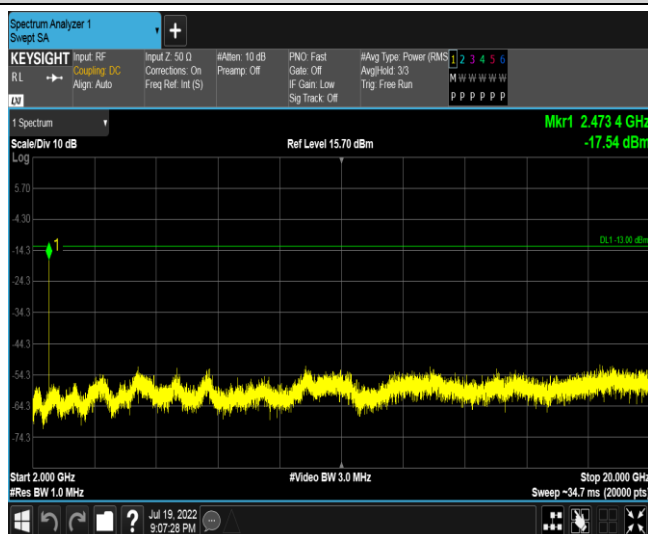
Band5-3MHz-QPSK-20415-1RB#0-Range3:2000~20000MHz
