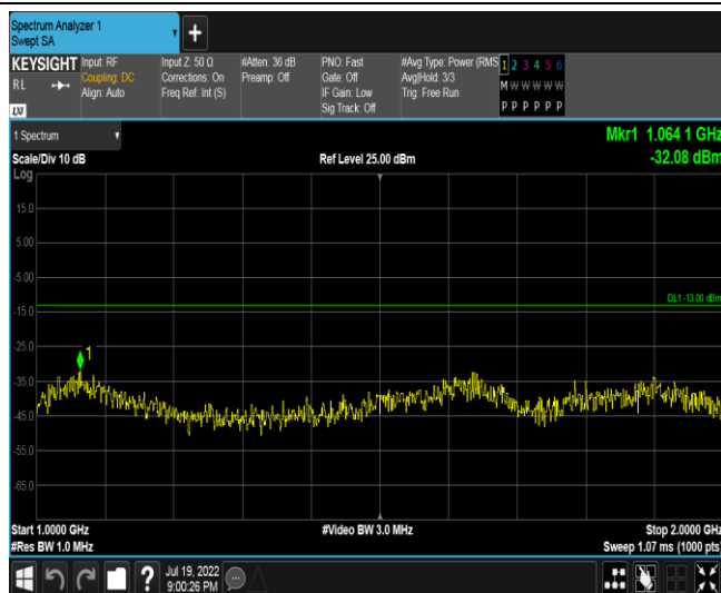
Band5-1.4MHz-16QAM-20407-1RB#0-Range5:1000~10000MHz
