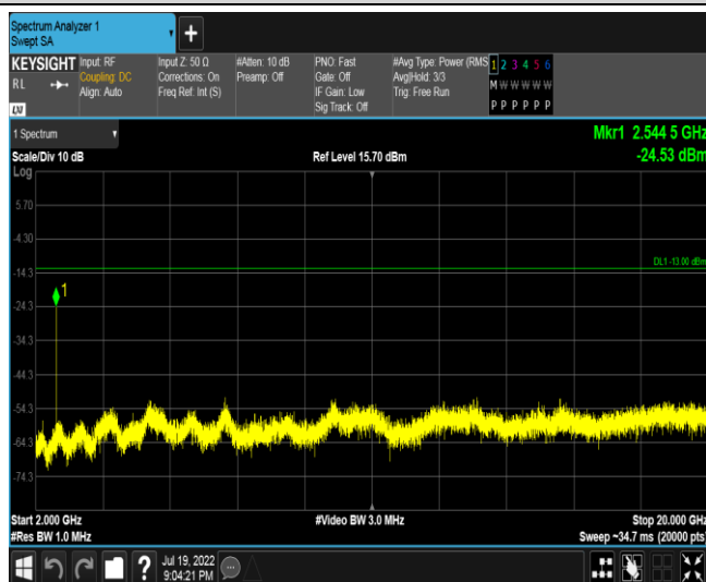
Band5-1.4MHz-QPSK-20643-1RB#0-Range3:2000~20000MHz
