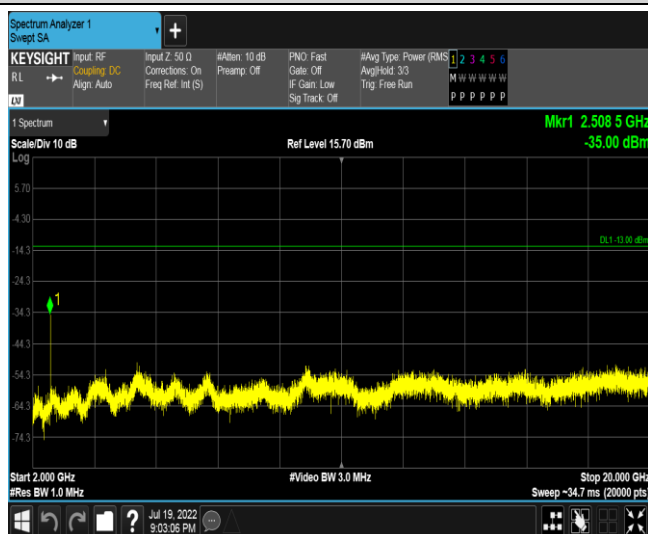
Band5-1.4MHz-16QAM-20525-1RB#0-Range3:2000~20000MHz
