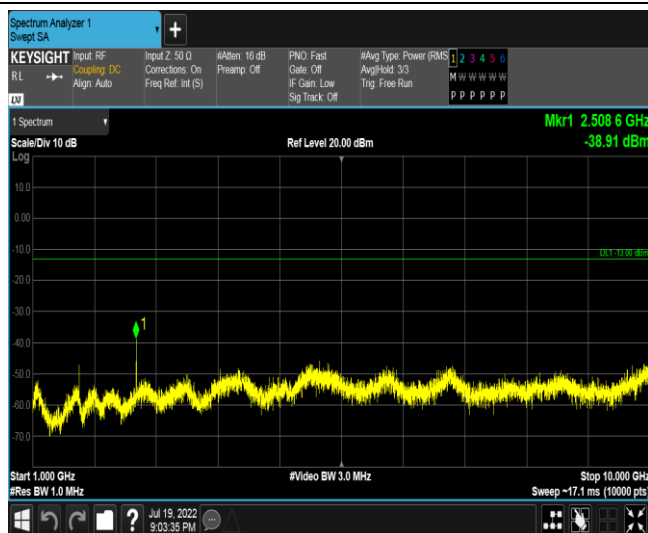
Band5-1.4MHz-16QAM-20525-1RB#0-Range2:1000~2000MHz
