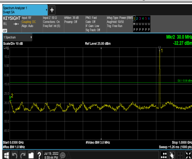
Band5-1.4MHz-QPSK-20407-1RB#0-Range1:30~1000MHz
