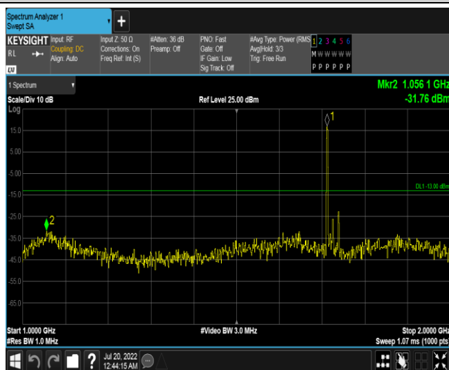
Band4-15MHz-16QAM-20025-1RB#0-Range2:1000~2000MHz
