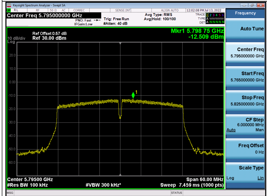
Test_Graph_802.11ac40_ANT1_5795_MCS9_PSD
